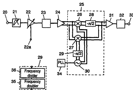
Fig. 1 23: second filter 24: unbalanced/balanced converter 25: image rejection mixer 29: phase shifter 31: balanced/unbalanced converter 32: intermediate frequency filter
