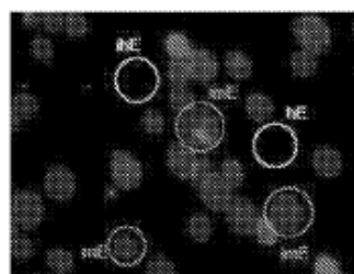
Immunofluorescence microscopy (TER-119: rodent erythrocytes)
