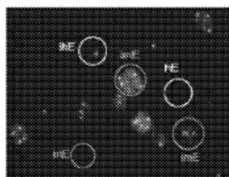
Immunofluorescence microscopy (DAPI : nuclei)
