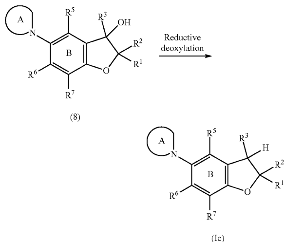
Reaction scheme 5
