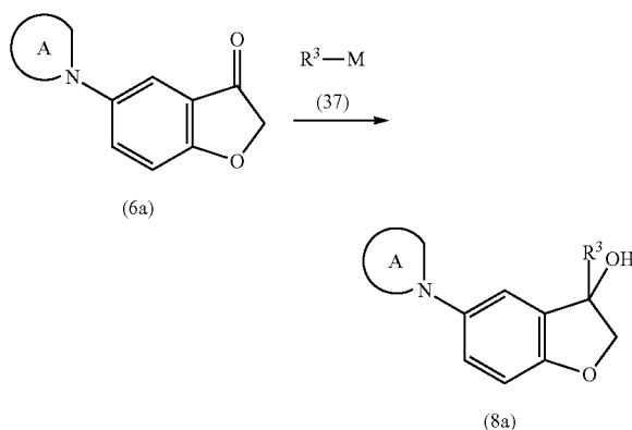
Reaction scheme 19
