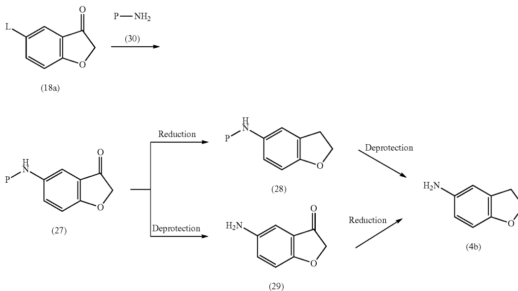
Reaction scheme 13
