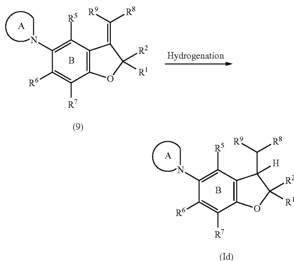
Reaction scheme 6
