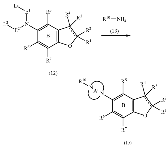
Reaction scheme 8
