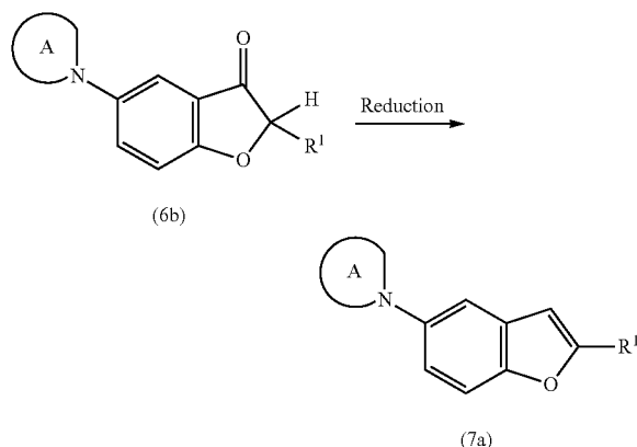
Reaction scheme 18
