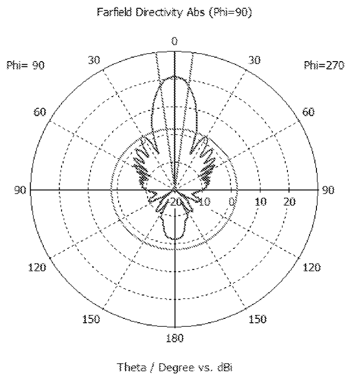
Antenna Gain Pattern
