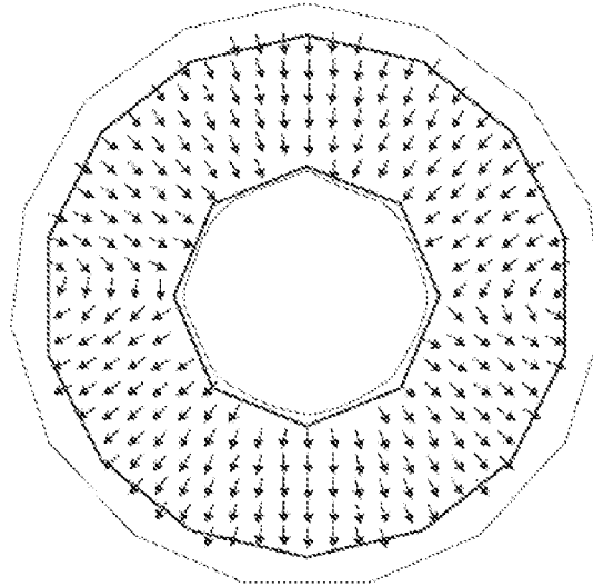
HE11, Horizontal Polarization
