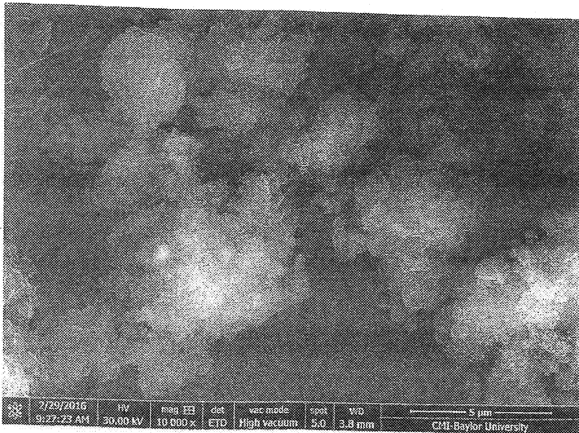
Figure 7. Scanning Electron micrograph of Ox65™ following nano-engineering. Magnification = 10,000x
