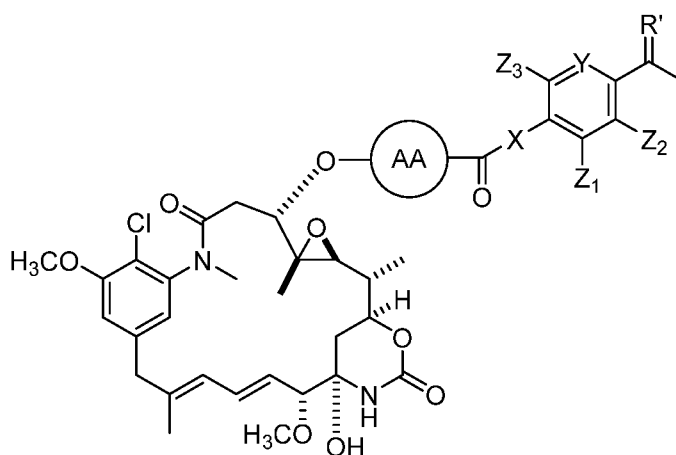
Formula (IV)
