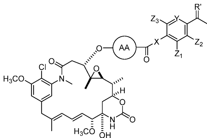
Formula (IV)
