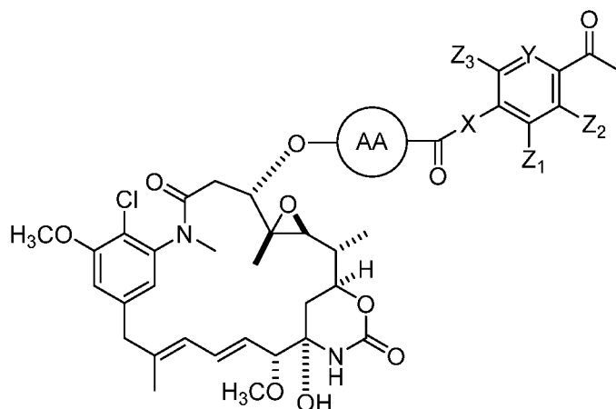
Formula (IV')
