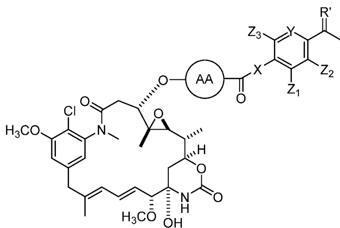
Formula (IV)
