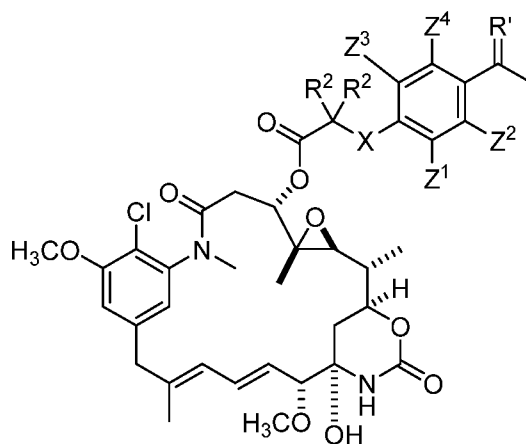
Formula (II)
