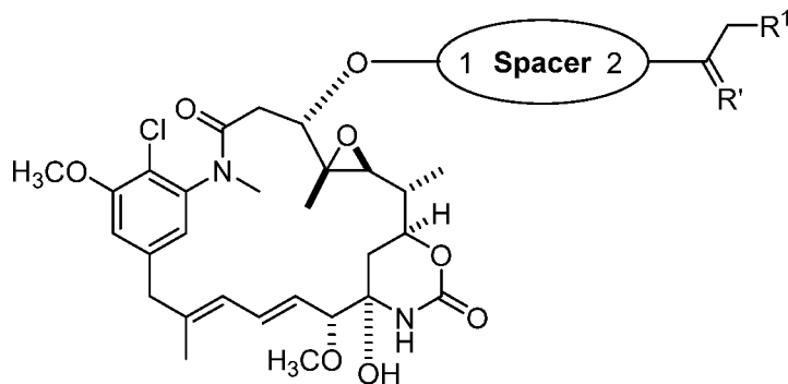
Formula (I)
