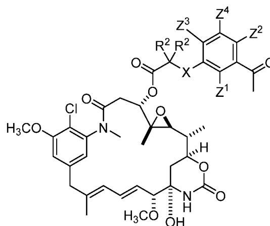
Formula (III')
