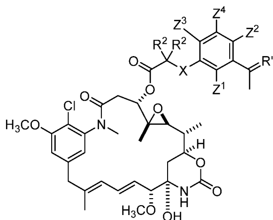
Formula (III)
