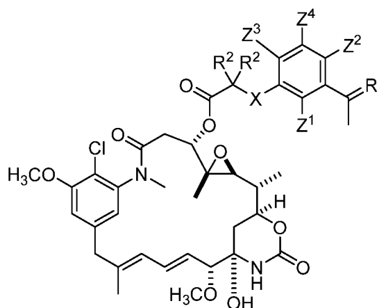
Formula (III)
