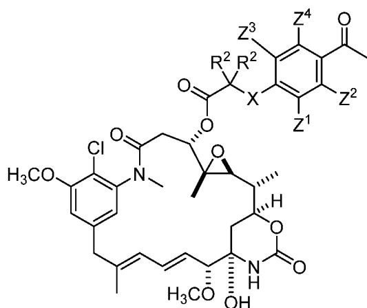
Formula (II')
