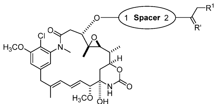
Formula (I)
