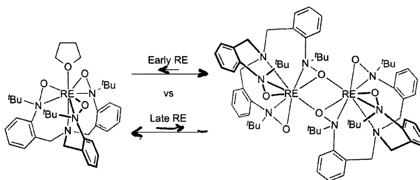
Scheme 1. Equilibrium between monomeric \text{RE}[(2-(^t\text{BuNO})\text{CH}_2-\text{C}_6\text{H}_4)_3\text{N}] complexes (i.e., 1-RE) and their dimeric \{\text{RE}[(2-(^t\text{BuNO})\text{CH}_2-\text{C}_6\text{H}_4)_3\text{N}]\}_2 analogs (i.e., 2-RE).
