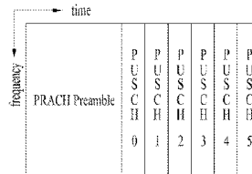
(b) TDM
