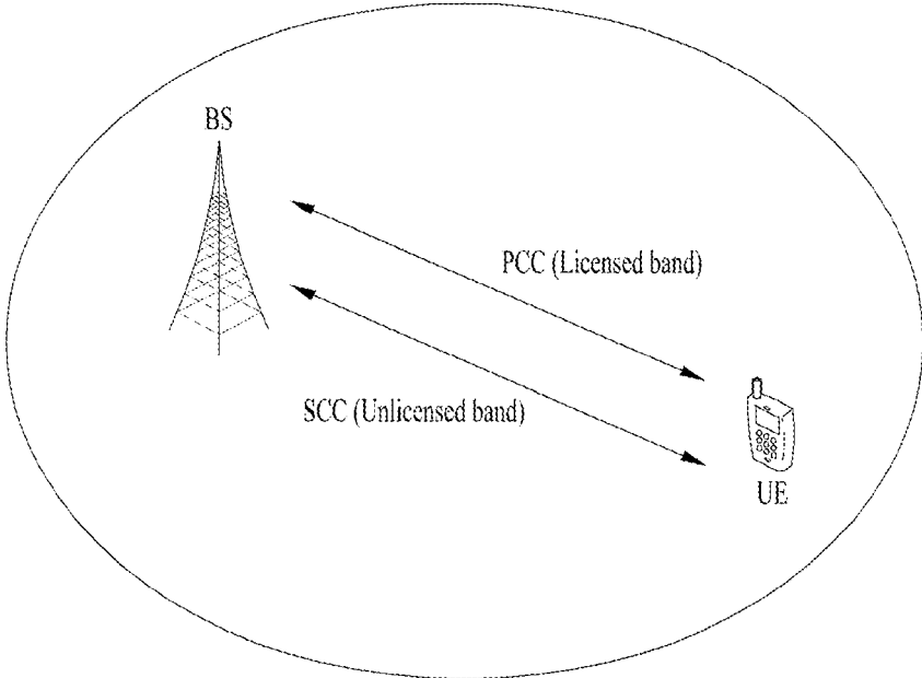
(a) Carrier aggregation between L-band and U-band
