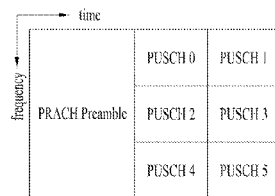
(c) FDM/TDM
