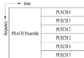
(a) FDM
