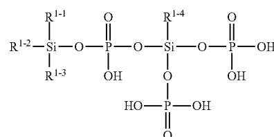
[Chemical Formula 61]
