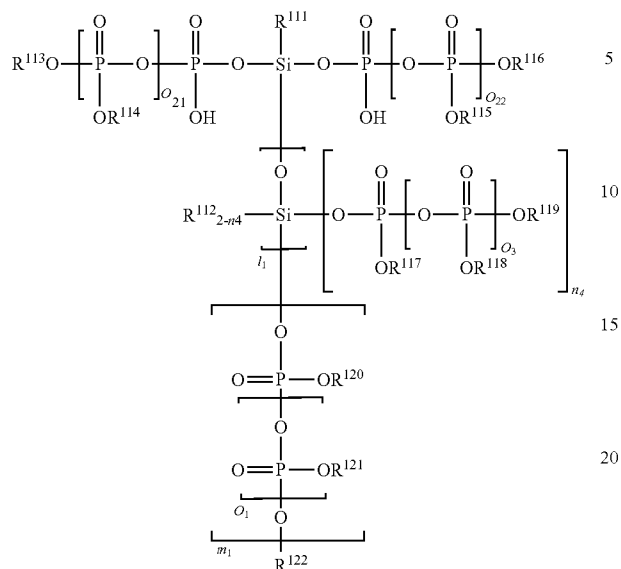
[Chemical Formula C200-1]
