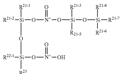
[Chemical Formula 265]
