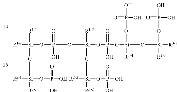
[Chemical Formula 210]
