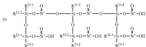
[Chemical Formula 269]
