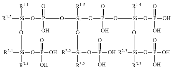
[Chemical Formula 209]
