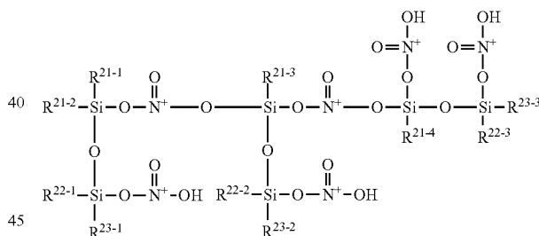
[Chemical Formula 269]
