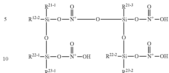
[Chemical Formula 267]
