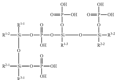
[Chemical Formula 208]
