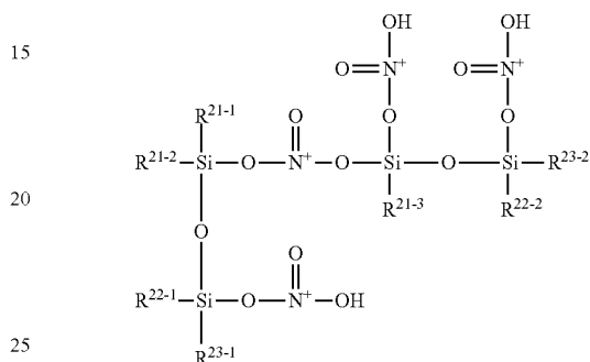
[Chemical Formula 268]
