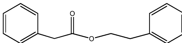
2-phenylethyl phenylacetate
