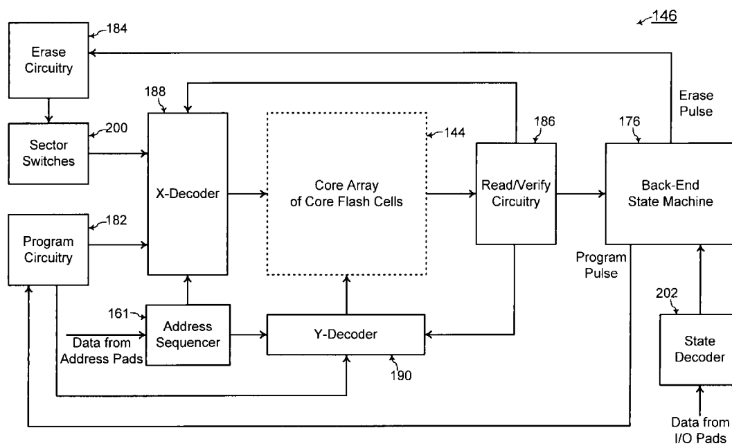
FIG. 7 (Prior Art)
