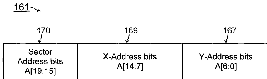
FIG. 9 (Prior Art)
