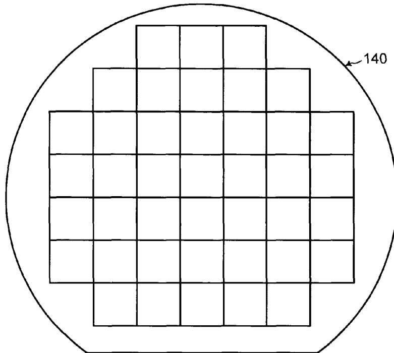
FIG. 4 (Prior Art)
