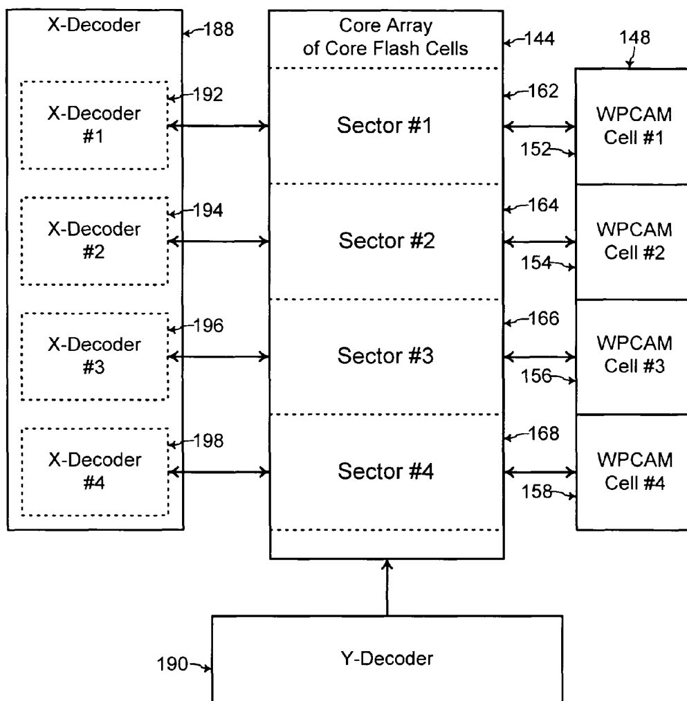
FIG. 8 (Prior Art)
