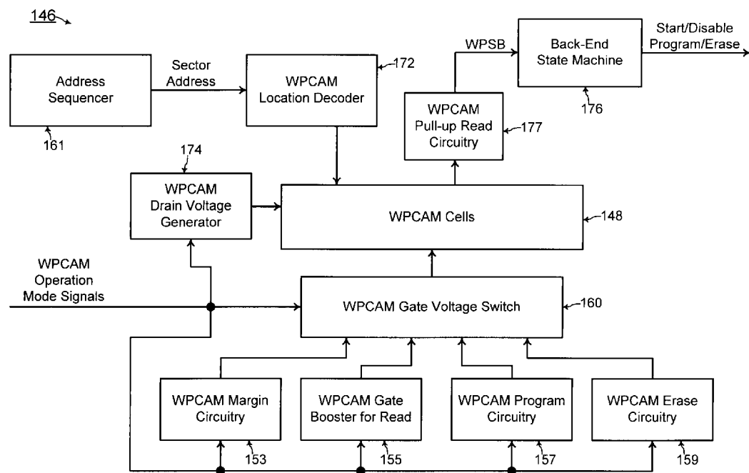
FIG. 6 (Prior Art)
