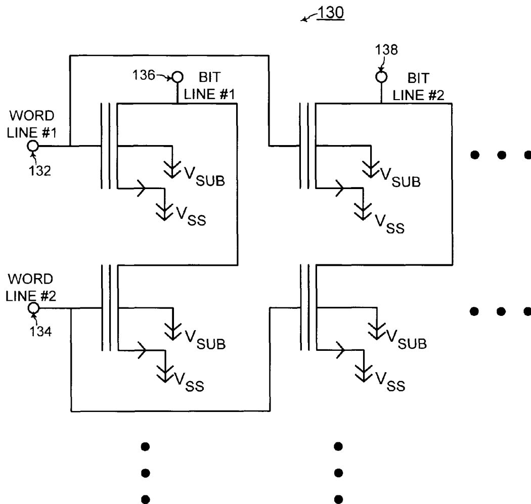
FIG. 3 (Prior Art)
