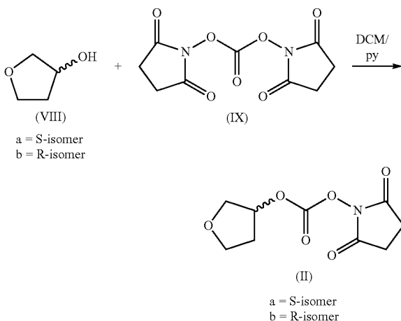
Scheme 5: process for preparation of (S)-3-tetrahydrofuranyl-N-succinimidyl carbonate
