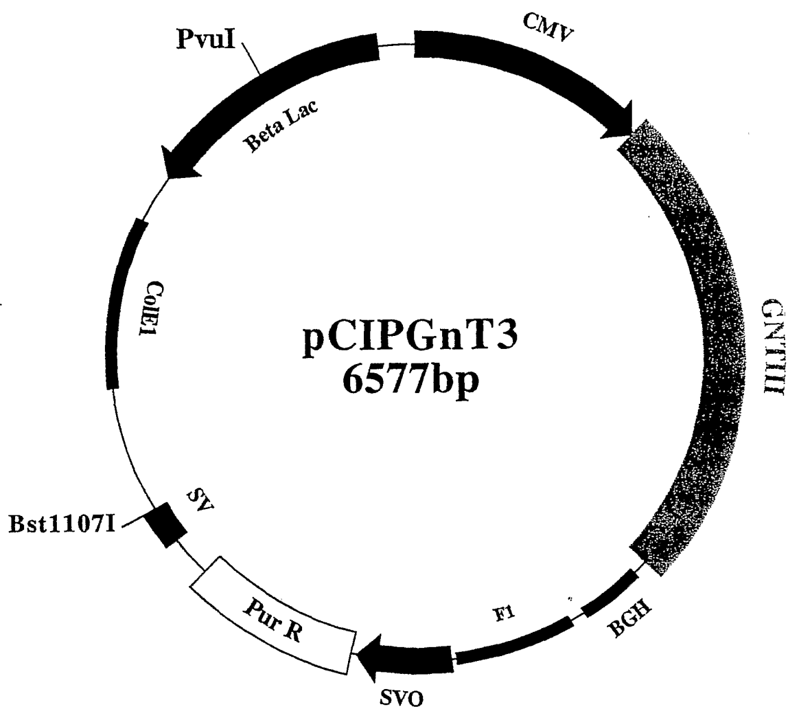
Figure 1 Plasmid pCIPGnT3
