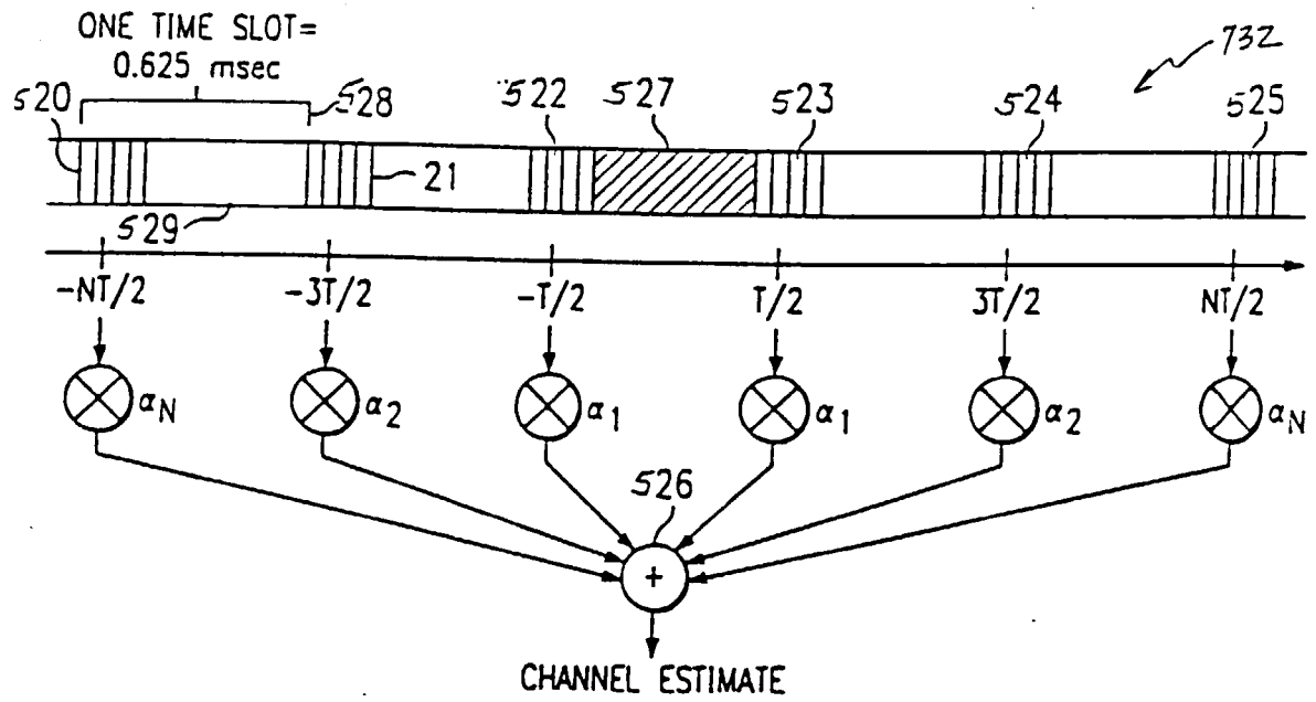
FIG. 5 (PRIOR ART)
