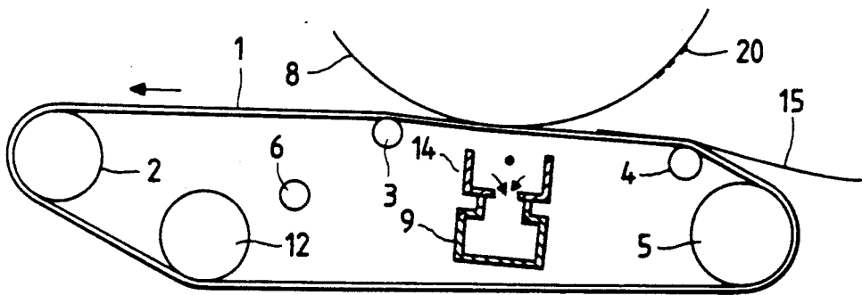
FIG. 4 PRIOR ART
