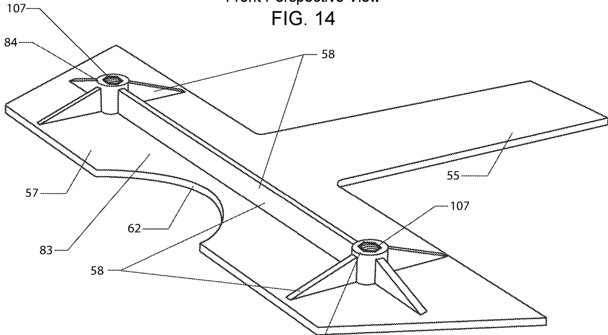
Kick Tail Mounting Plate With Tongue With Leash Pin Cut Out Front Perspective View
