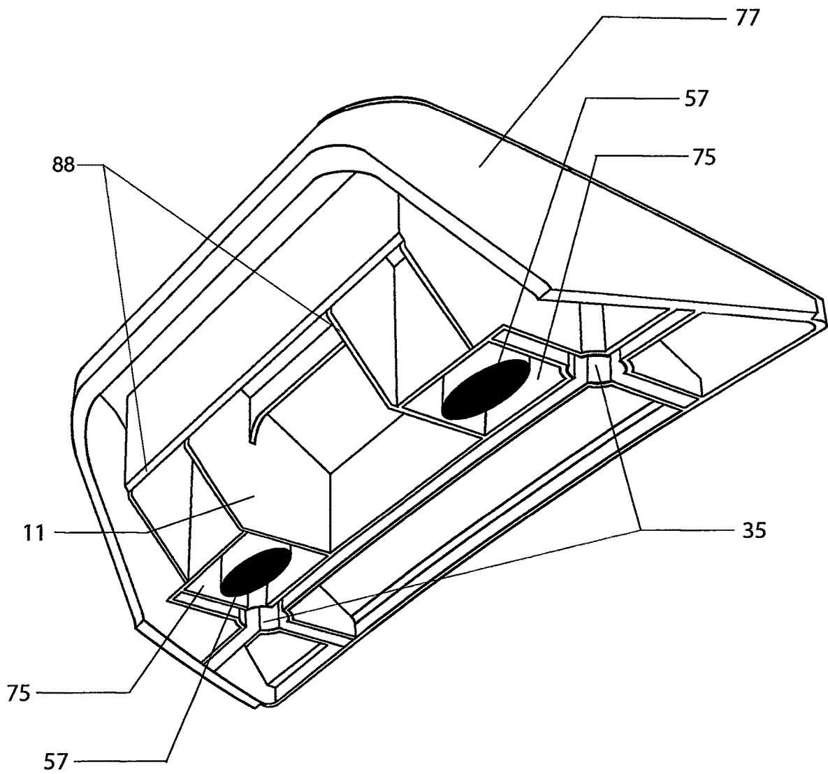
Hollow Skateboard and Surfboard Kick Tail With Ramp To Flat Top Bottom Perspective View FIG. 17
