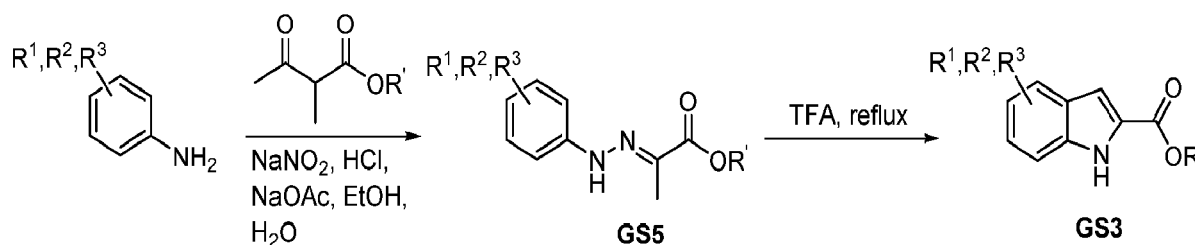
Scheme 2
