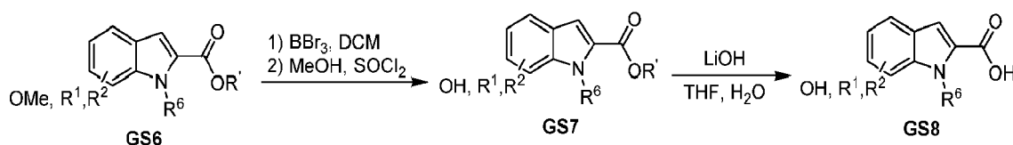
Scheme 3
