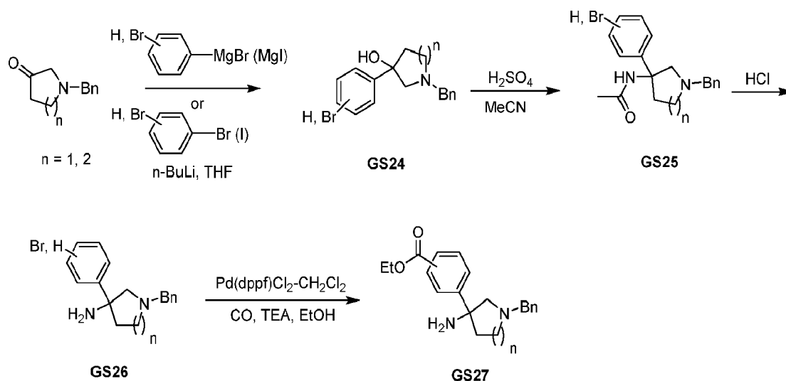
Scheme 9
