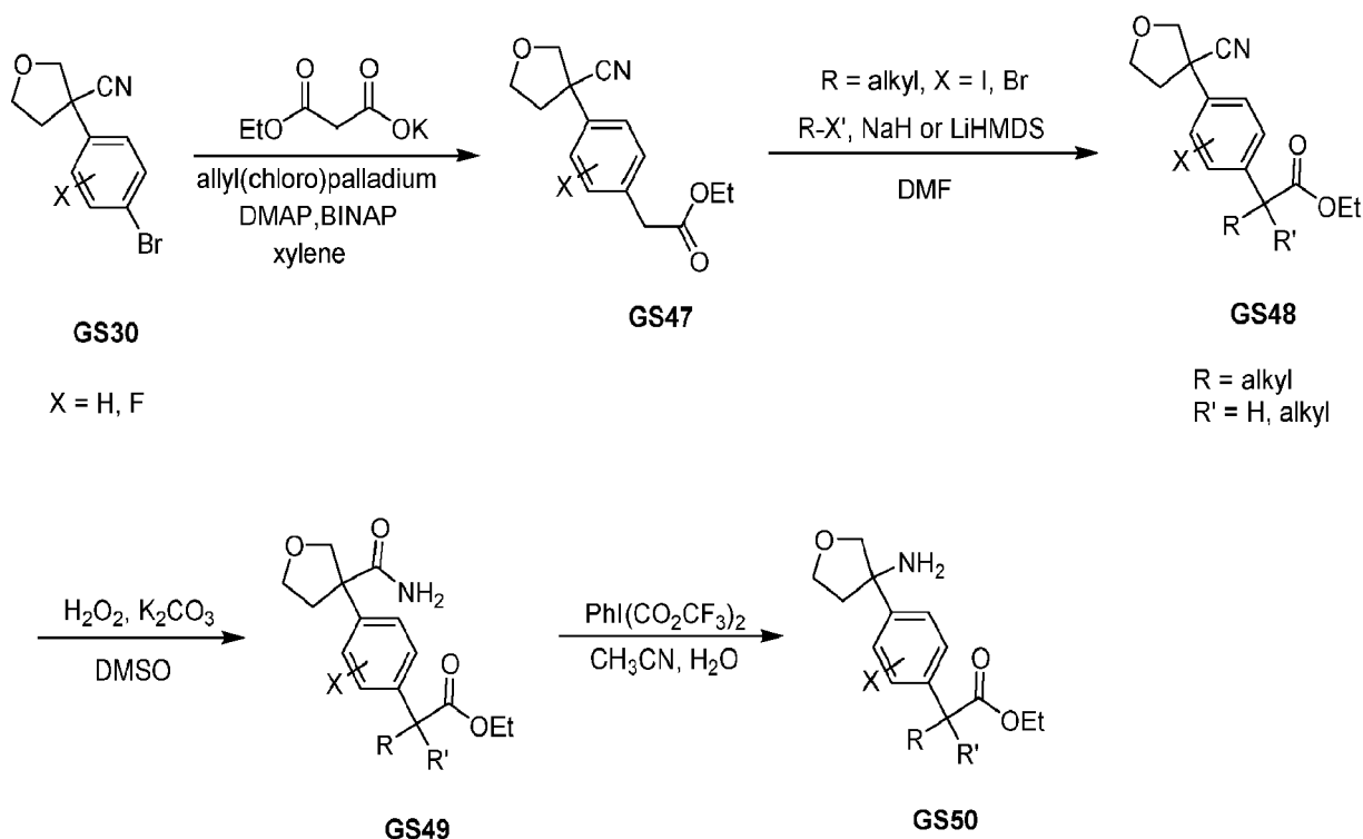
Scheme 14
