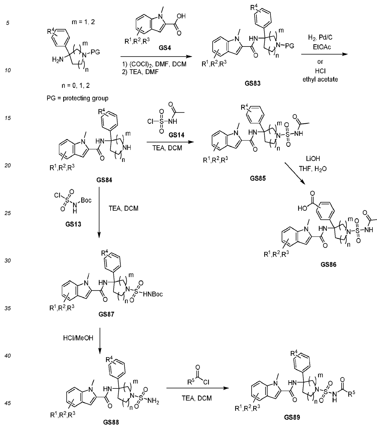
Scheme 24
