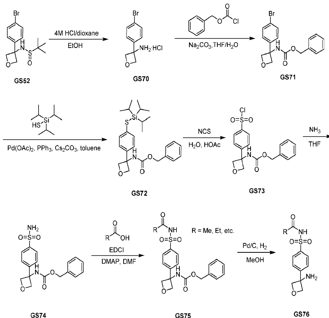
Scheme 20
