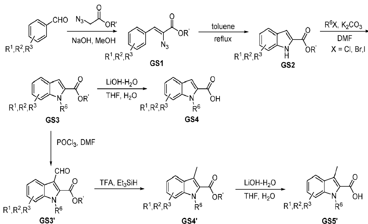
Scheme 1
