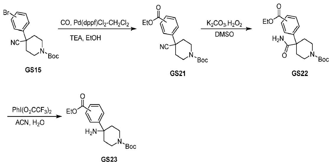
Scheme 8
