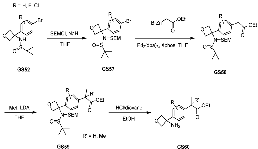
Scheme 17
