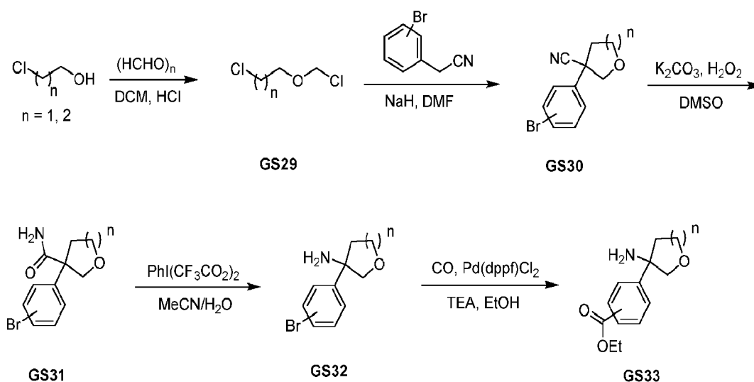
Scheme 10
