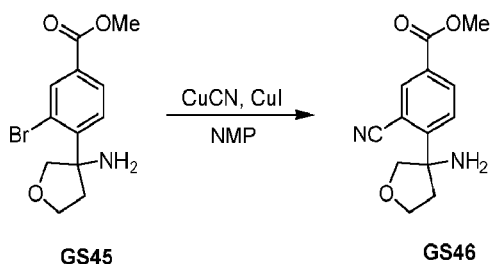
Scheme 13
