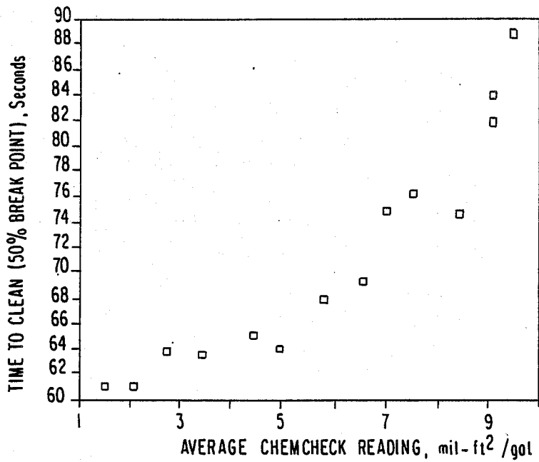
DEVELOPING TIME VERSUS LOADING
