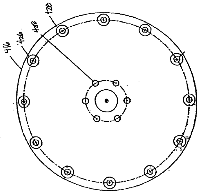
VIEW C-C FIG. 18A
