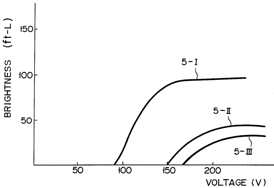
FIG. 5 (PRIOR ART)
