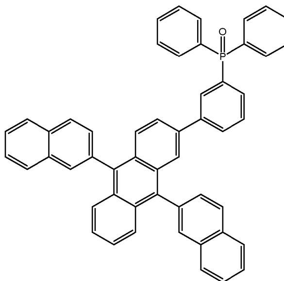
Chemical Formula 4
