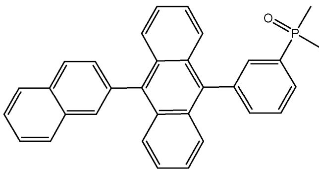
Chemical Formula 4
