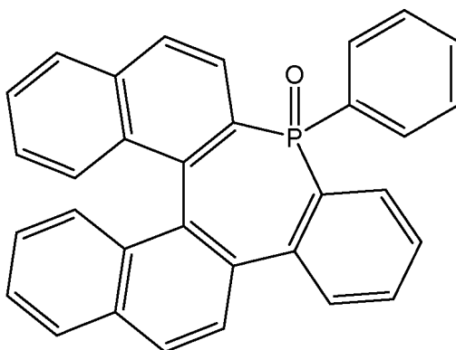
Chemical Formula 2
