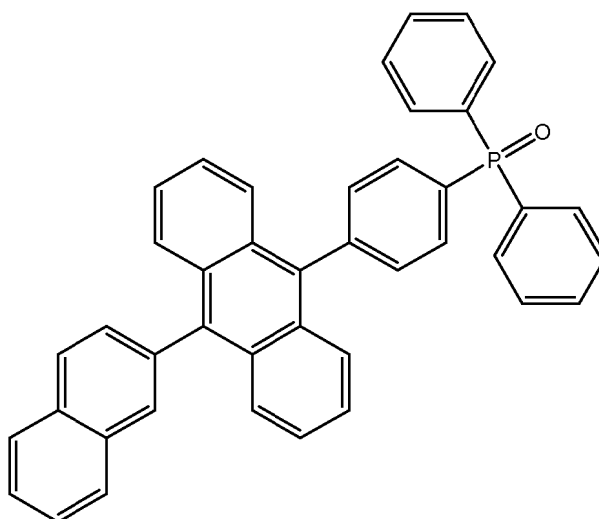
Chemical Formula 2
