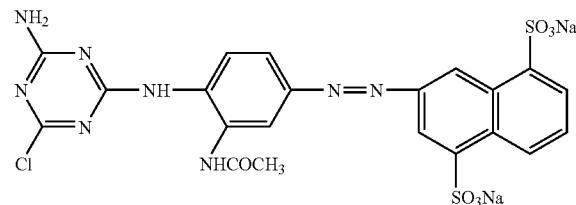
C.I. Reactive Yellow 3
