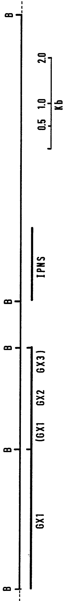
Fig. 6(a) FLAVOBACTERIUM DNA (II)
