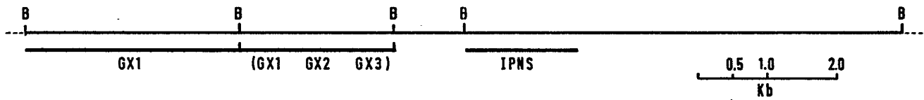
Fig. 6(a) FLAVOBACTERIUM DNA (II)
