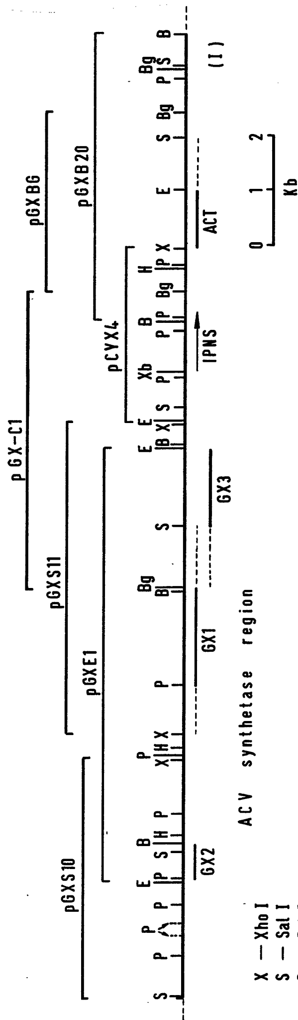
Fig. 6(b) P. CHRYSOGENUM DNA (I) IN pCX3.2
