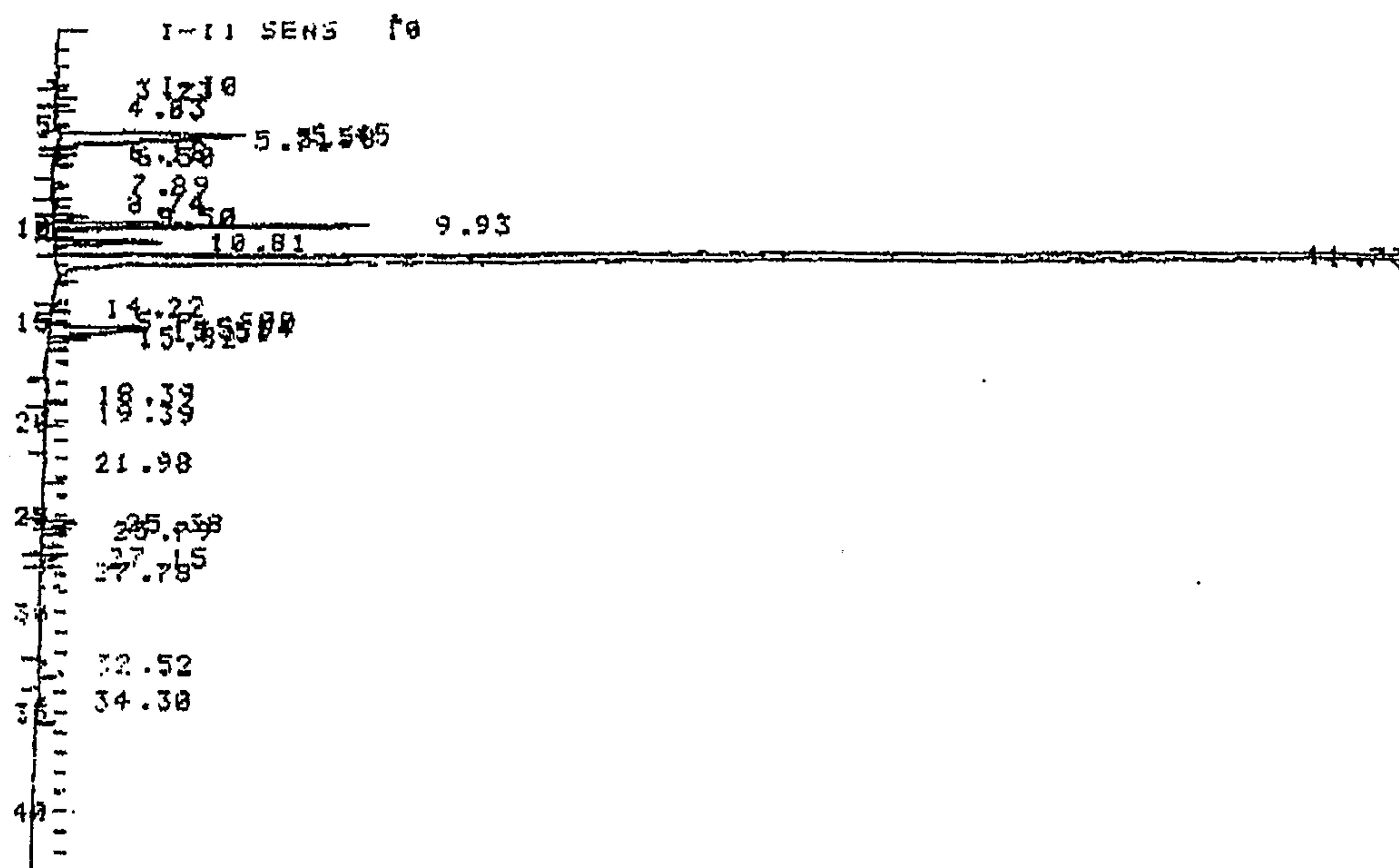
Figure 1. HPLC chromatogram of Compound VI.
