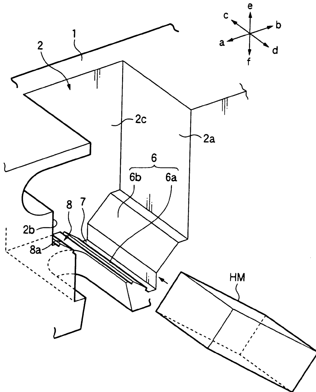
FIG.11 PRIOR ART
