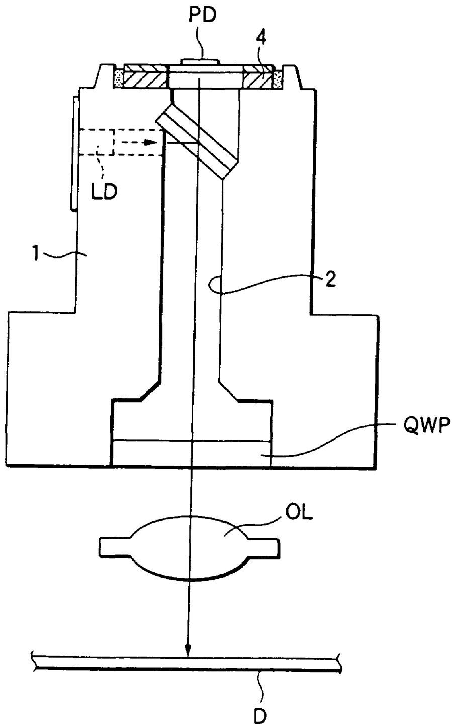
FIG.8 PRIOR ART
