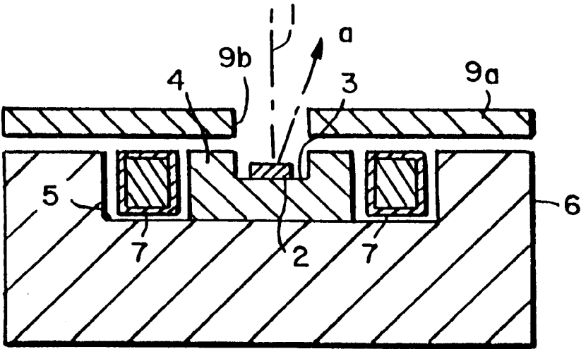
FIG. 1 PRIOR ART
