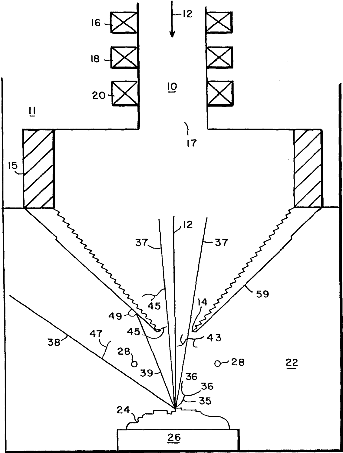
FIG. 4 PRIOR ART
