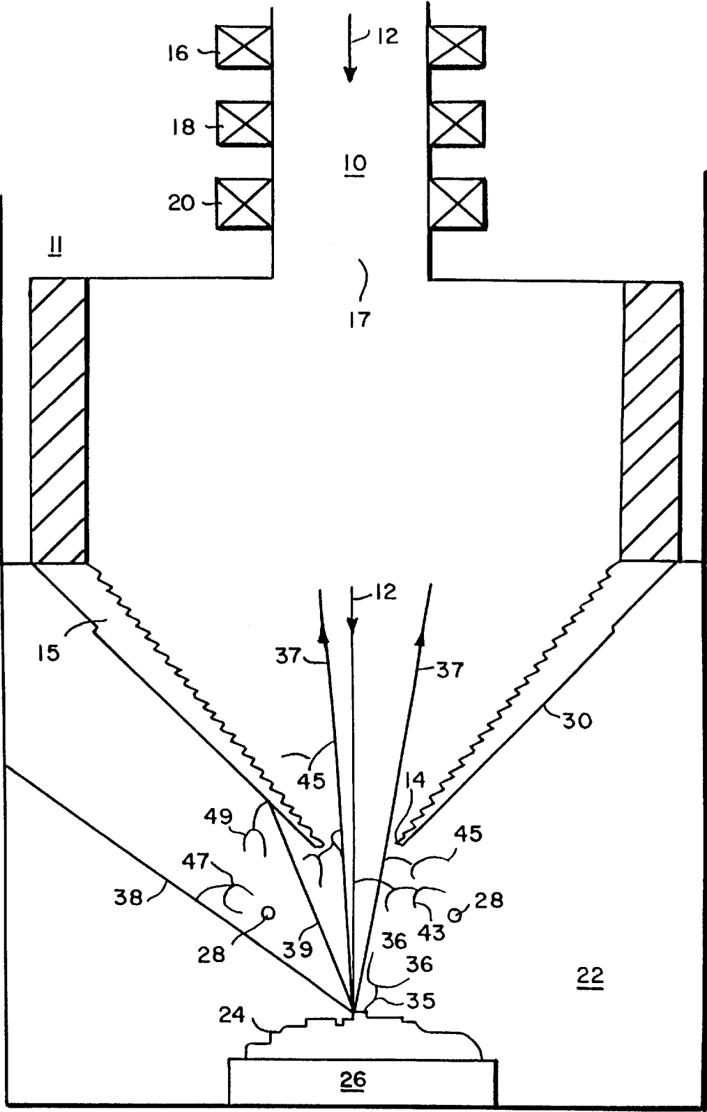
FIG. 3 PRIOR ART
