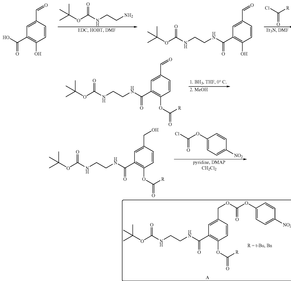
Scheme 12. Synthesis of the esterase cleavable linker.
