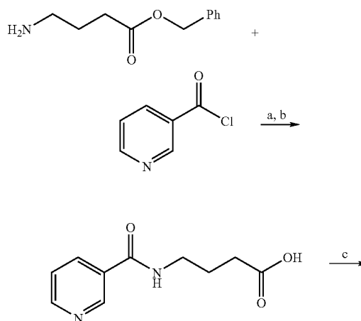
Scheme 4. Synthesis of locking module.
