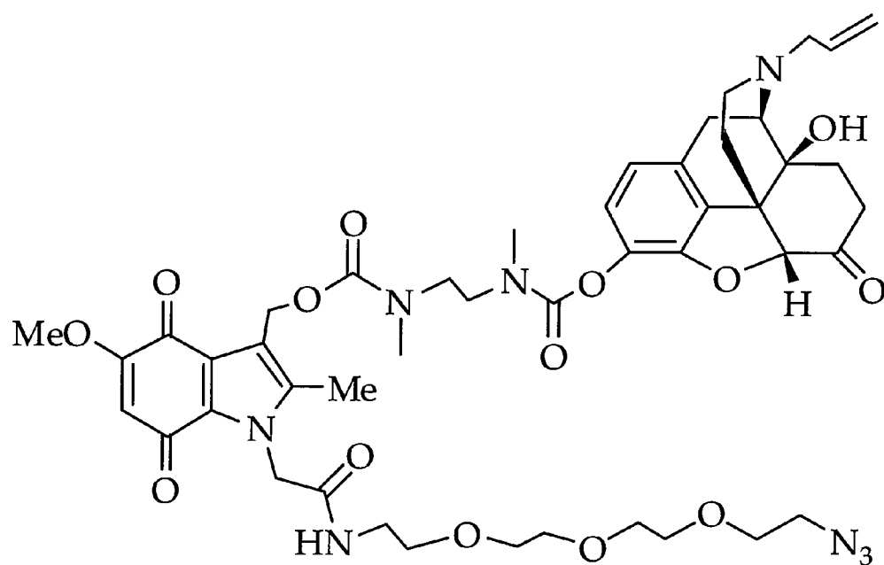
Indolequinone-based Naloxone Pro-drug
