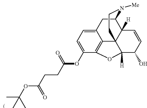
Prodrug A Aliphatic ester
