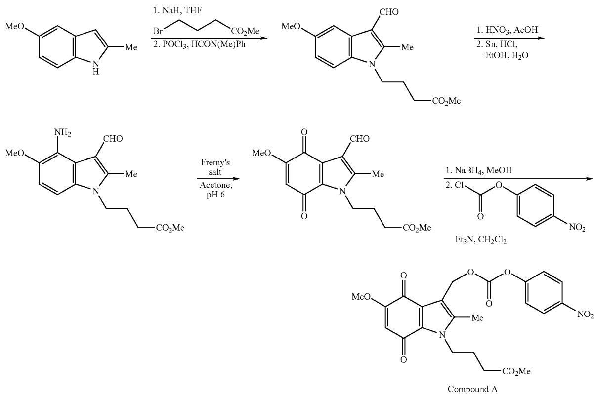
Scheme 9. Synthesis of the indoquinone-Naloxone linker.
