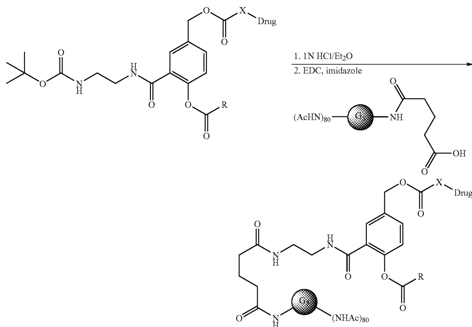
Scheme 14. Drug-linker conjugation to dendrimer.
