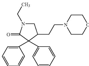
Scheme 3. Molecular structure of Doxapram
