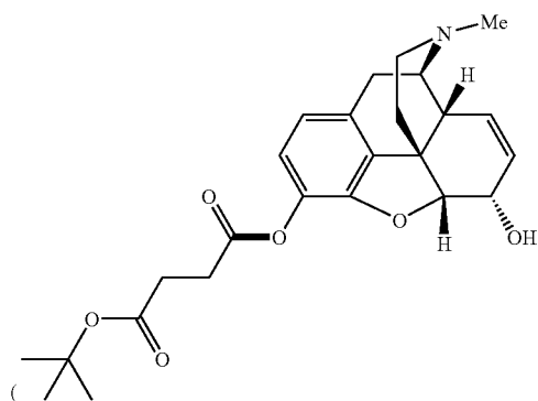
Prodrug A Aliphatic ester
