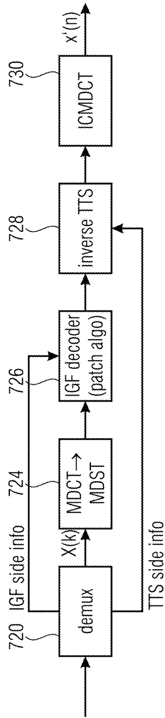
FIG 7B (DECODER)
