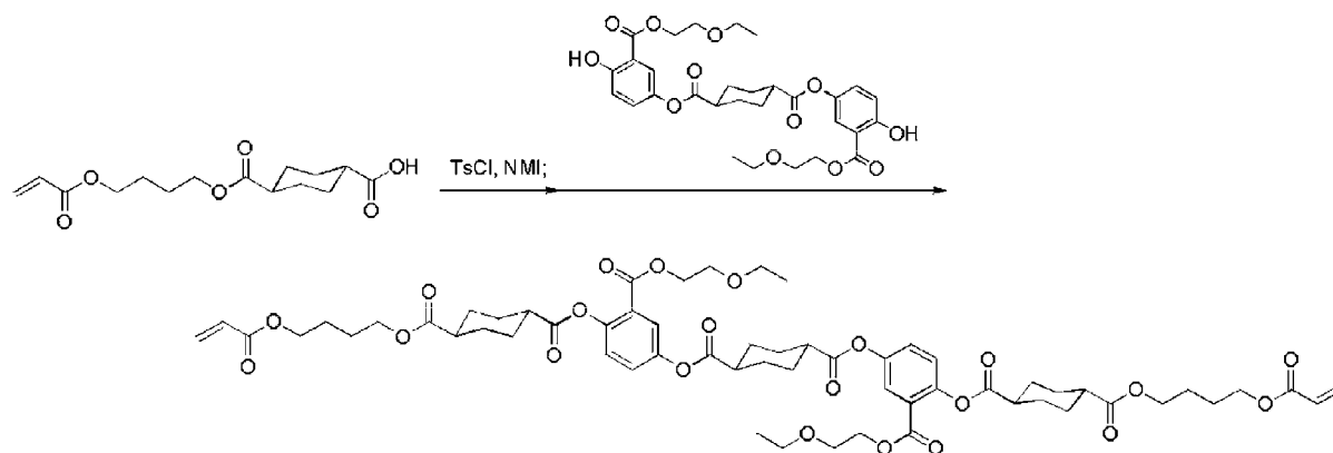
Compound 1
