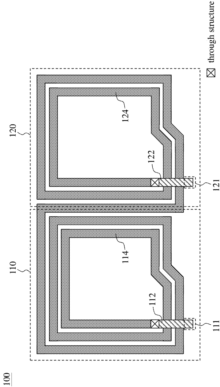
Fig. 1 (prior art)
