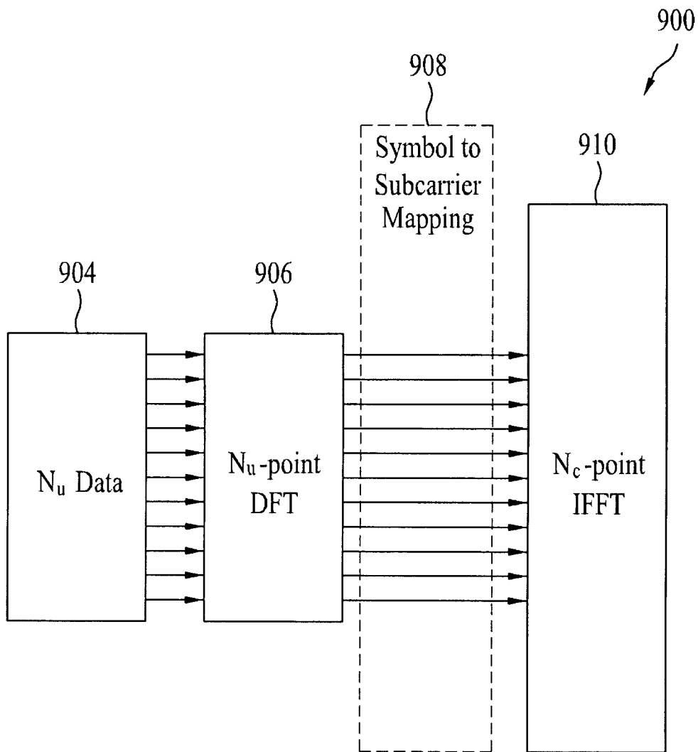
Localized DFT-s-OFDMA
