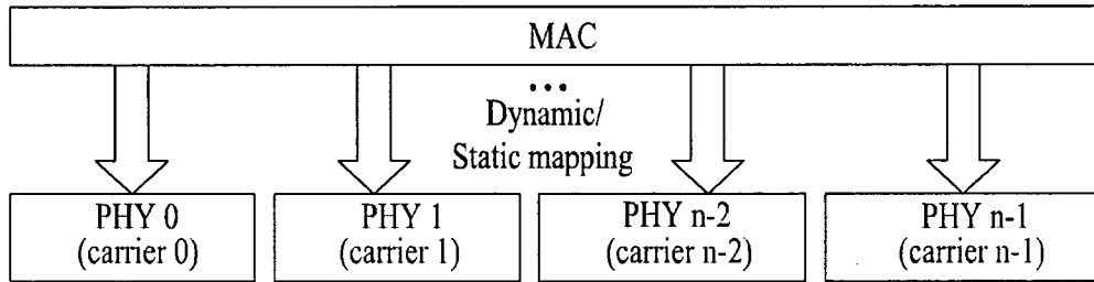
(a) Transmitter
