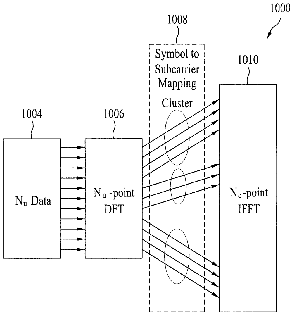
Clustered DFT-s-OFDMA
