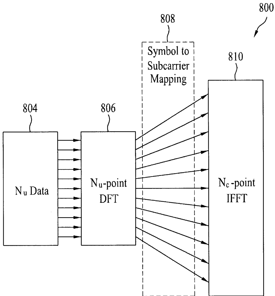
Interleaved DFT-s-OFDMA
