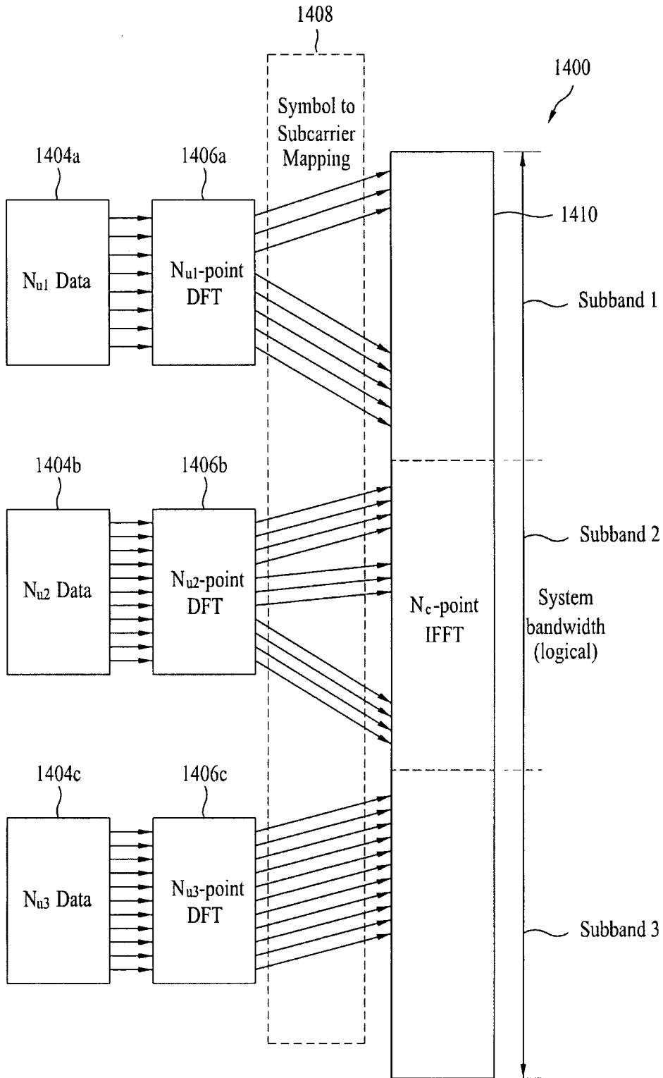
Another example of hybrid N_x /clustered DFT-s-OFDMA transmitter
