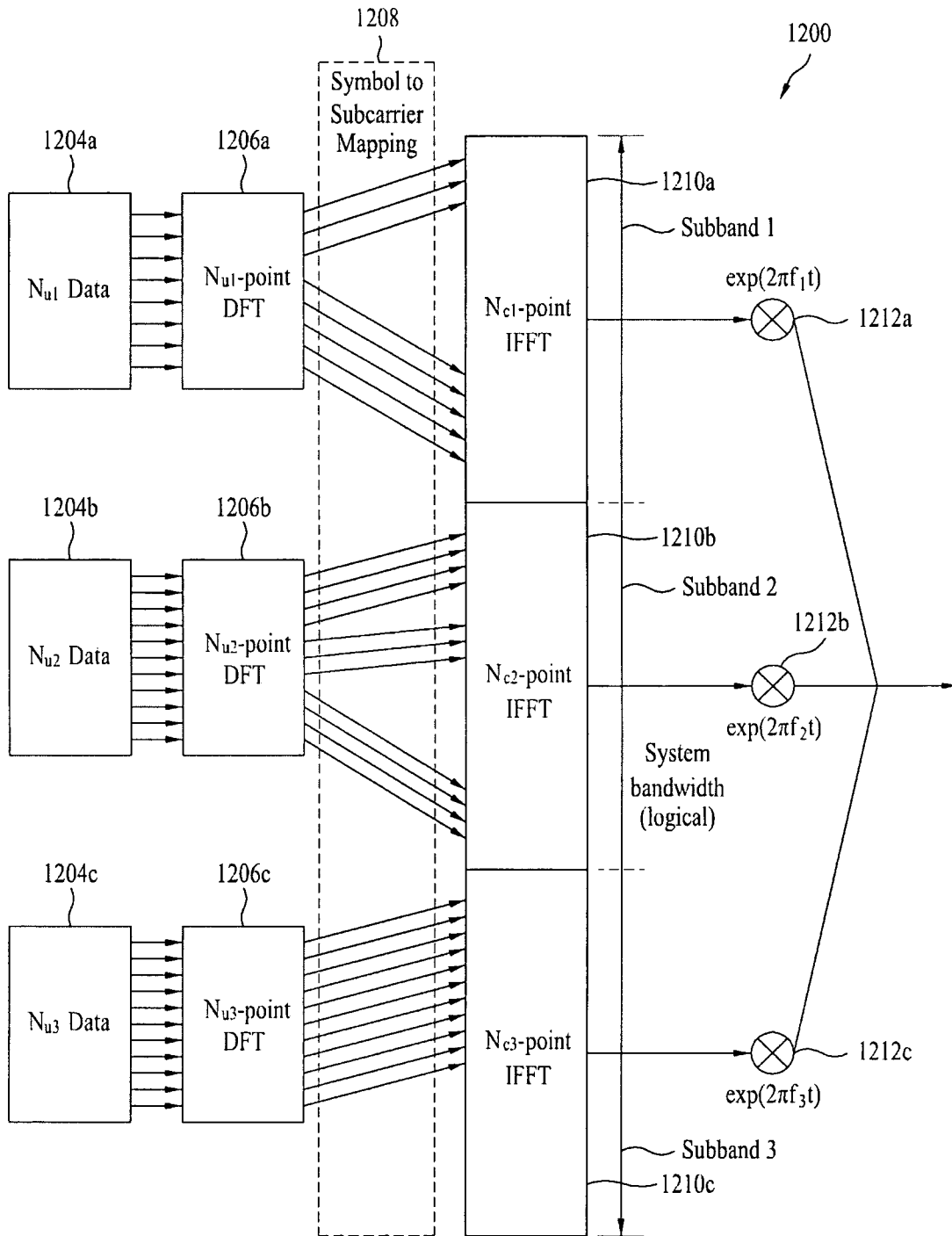
Another example of hybrid N_x /clustered DFT-s-OFDMA transmitter
