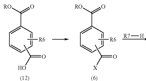
Reaction scheme 2:
