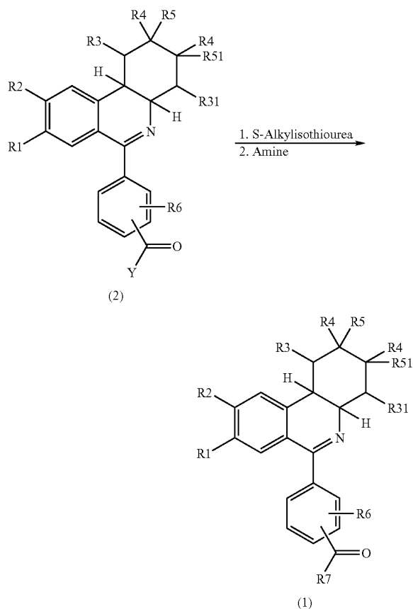
Reaction scheme 2:
