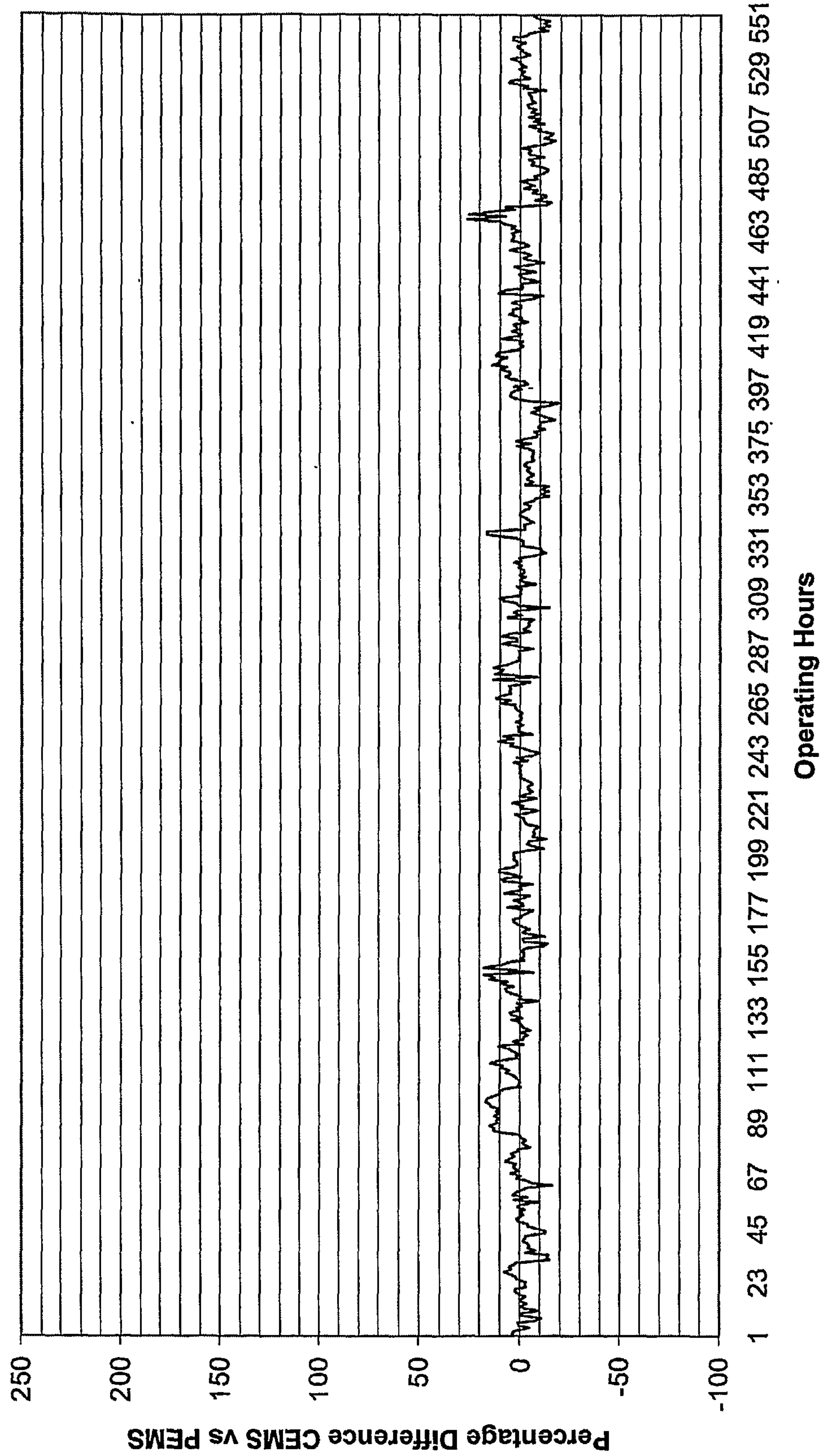
Figure 8: time plot of differences between predicted and measured NOx emissions (Example: 170 MW Combined Cycle Gas Turbine)
