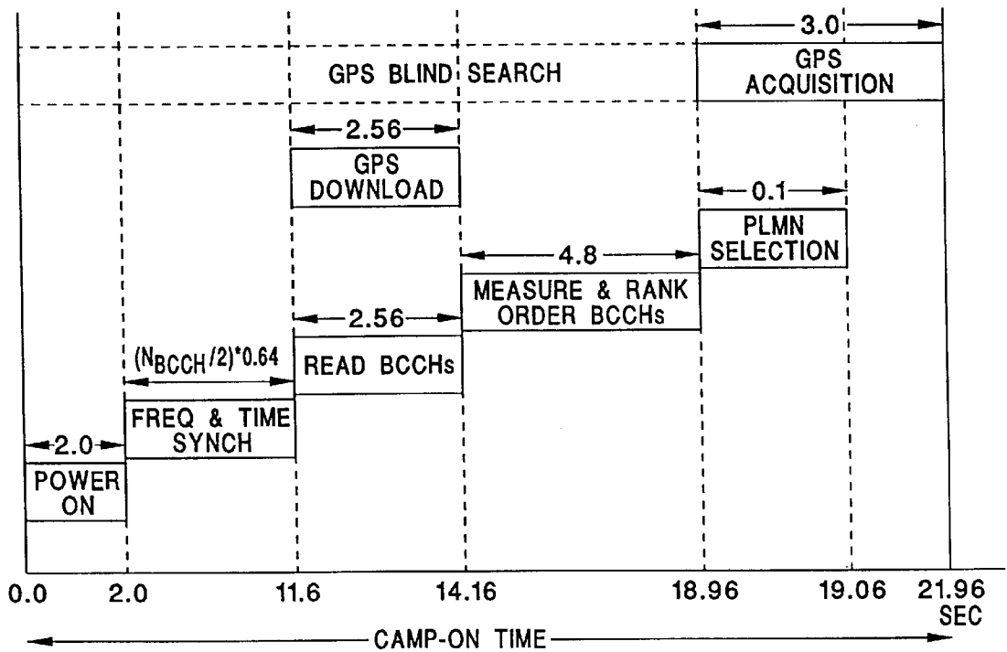
CAMP-ON TIME FOR COLD START WHEN N_{BCCH}=30
