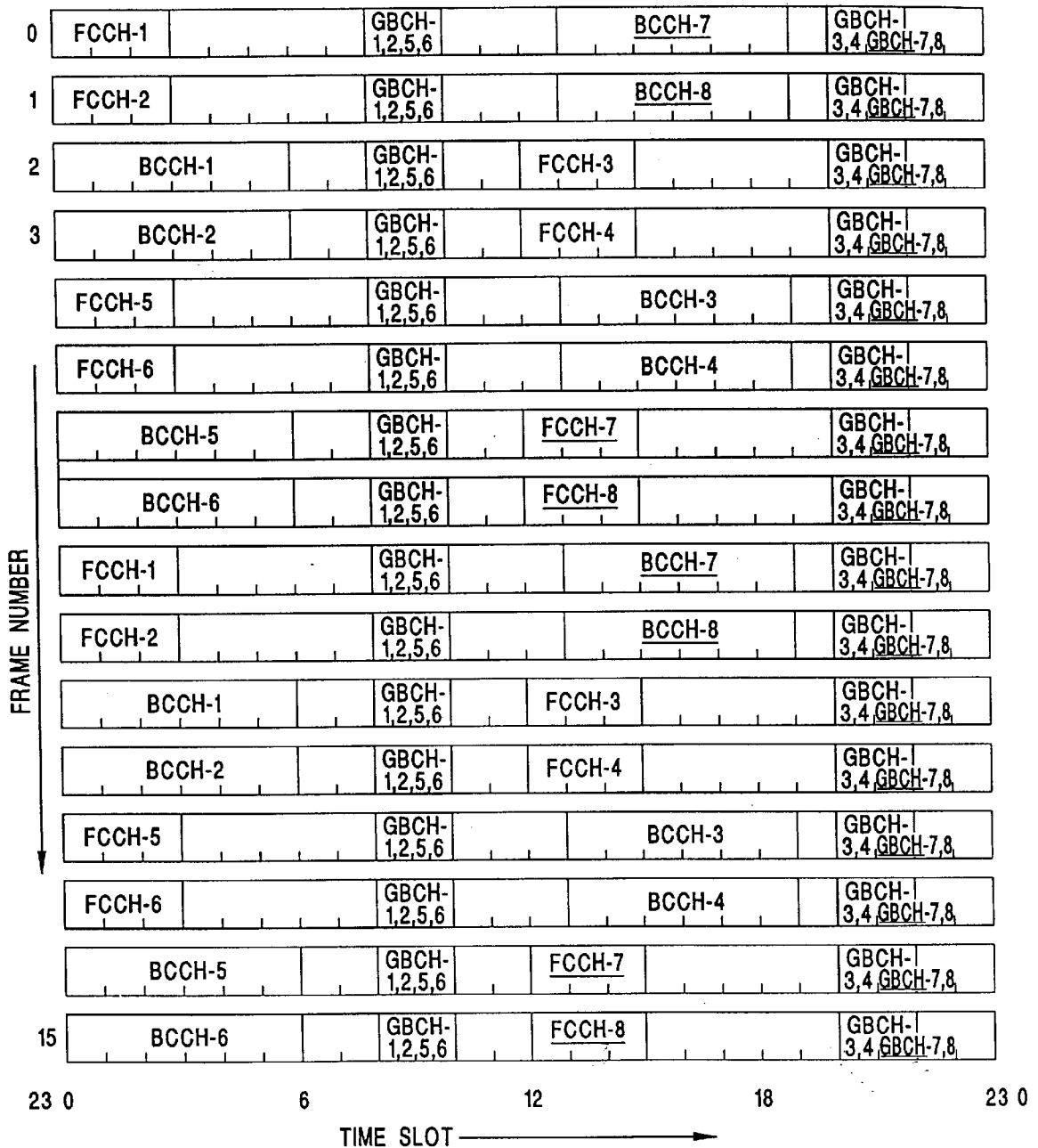
FHCHs AND BCCH POSITIONS WITHIN A MULTIFRAME BETWEEN TWO REGIONS
