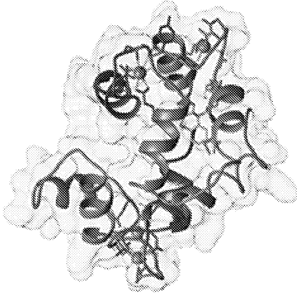
Bound to Ca 2+ and TFP
