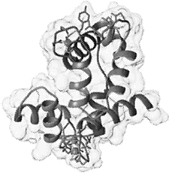
Bound to Ca 2+ and M13
