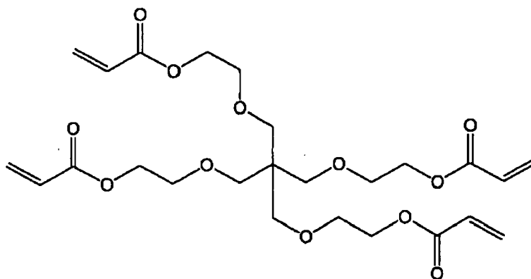
KAYARAD RP-1040 (manufactured by Nippon Kayaku Co., Ltd.)
