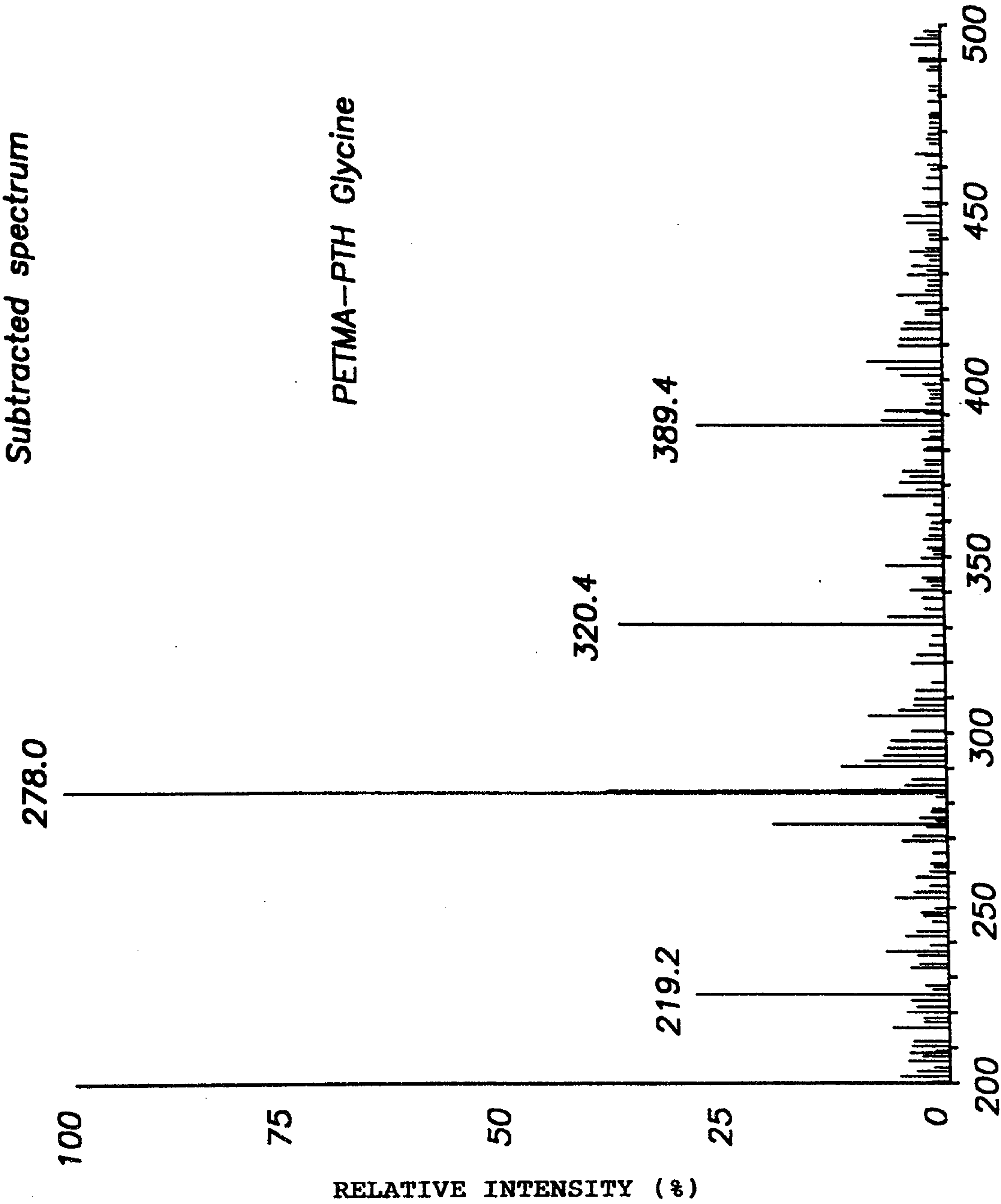
Figure 3 m/z
