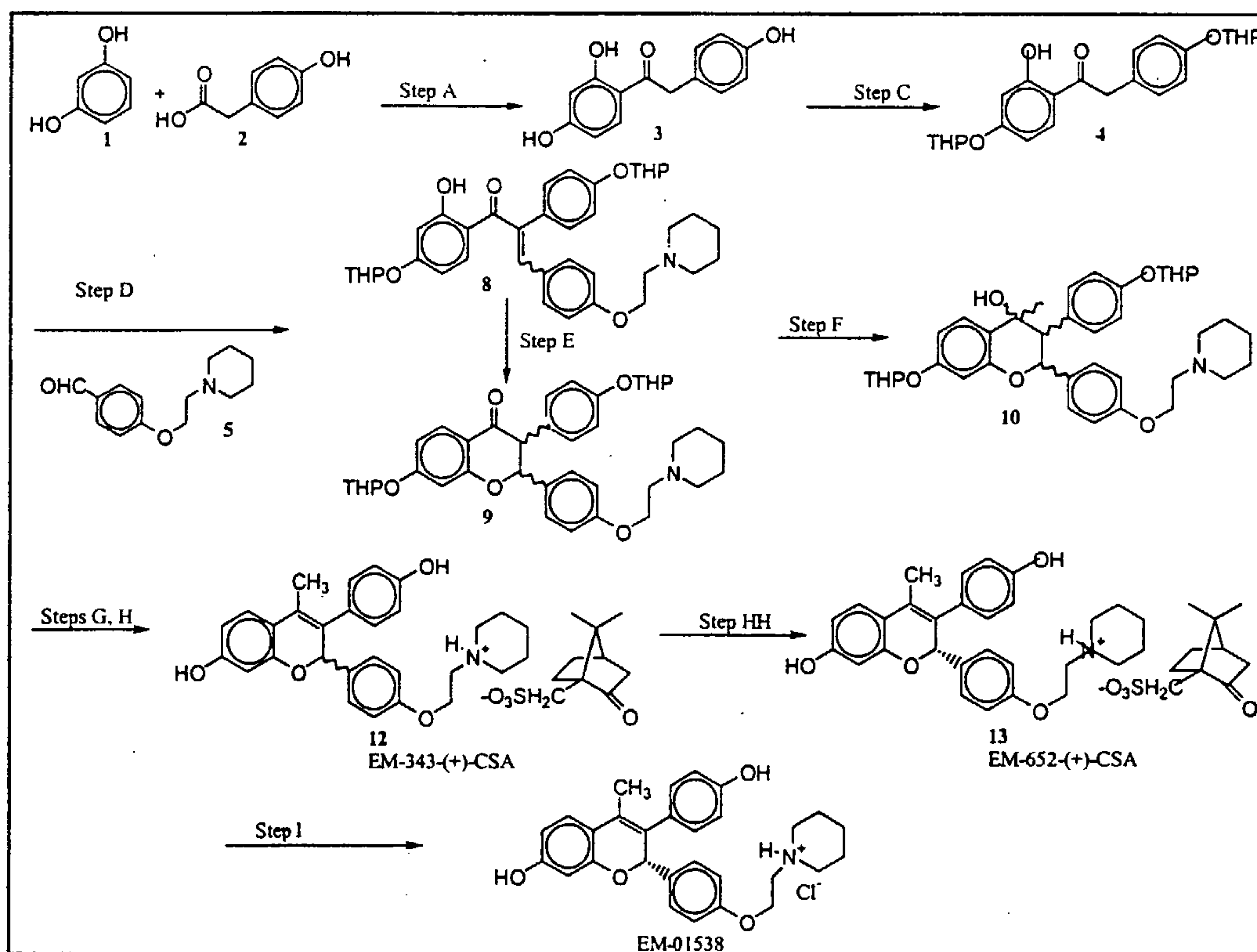
Scheme 1
