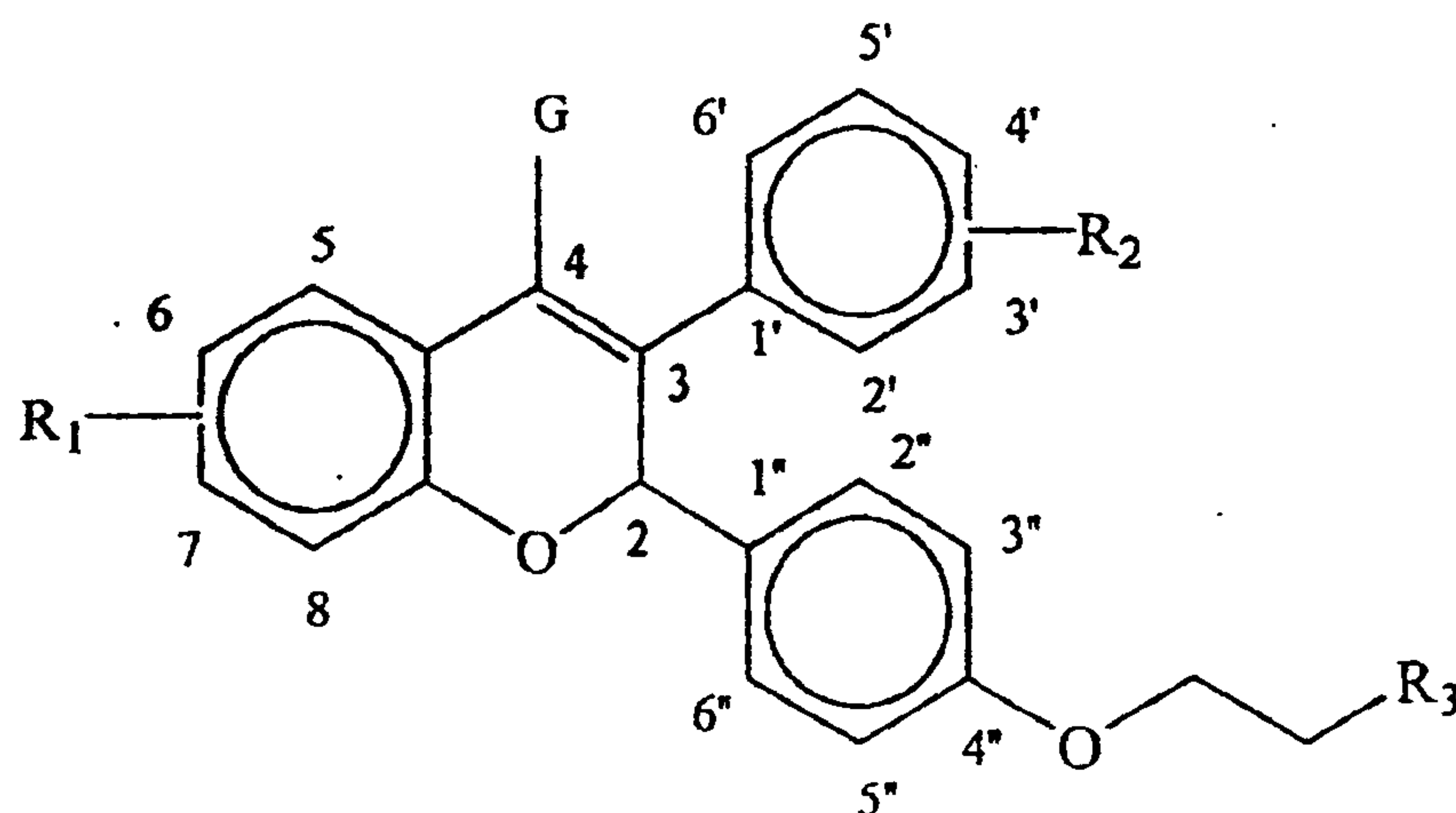
Formula I
