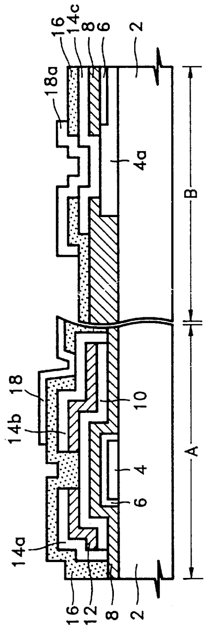
FIG. 5 (PRIOR ART)
