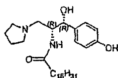
D-threo-4'-hydroxy-P4
