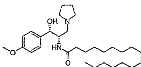
DL-threo (reference)
