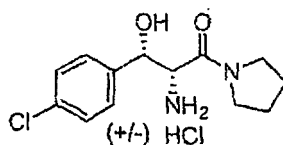
Compound 14
