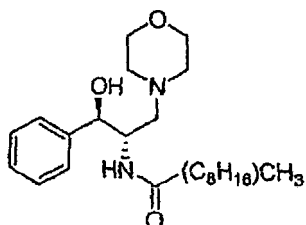
DL-erythro-PDMP
