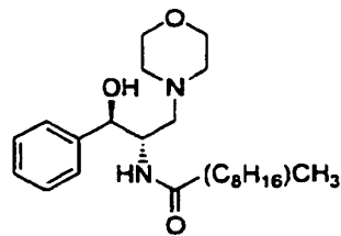
DL-erythro-PDMP
