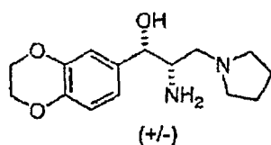
Compound 6
