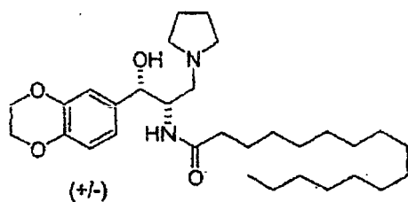
Compound 8
