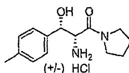
Compound 17
