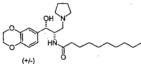
Compound 7
