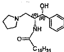
D-threo-P4
