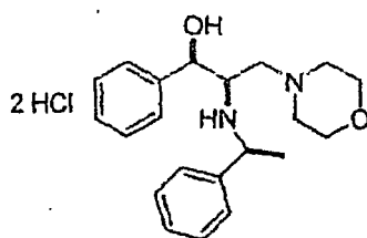
Compound 5
