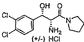
Compound 15
