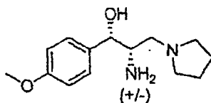
Compound 9
