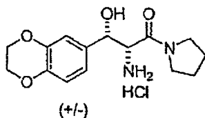
Compound 12
