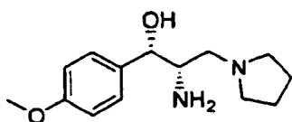
DI-threo
