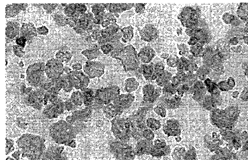
Sample 2-H (6.65%), 200X after retort simulation
