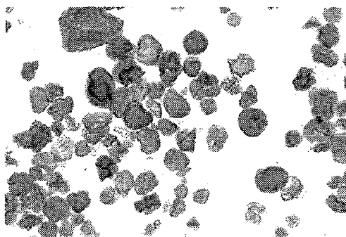
Sample 2-F (6.65%), 200X after retort simulation
