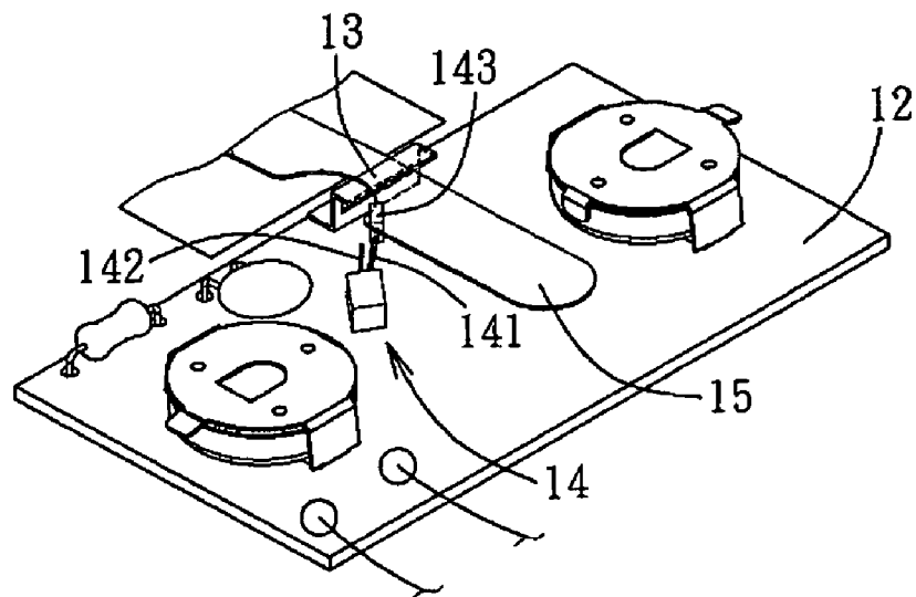
FIG. 3 PRIOR ART
