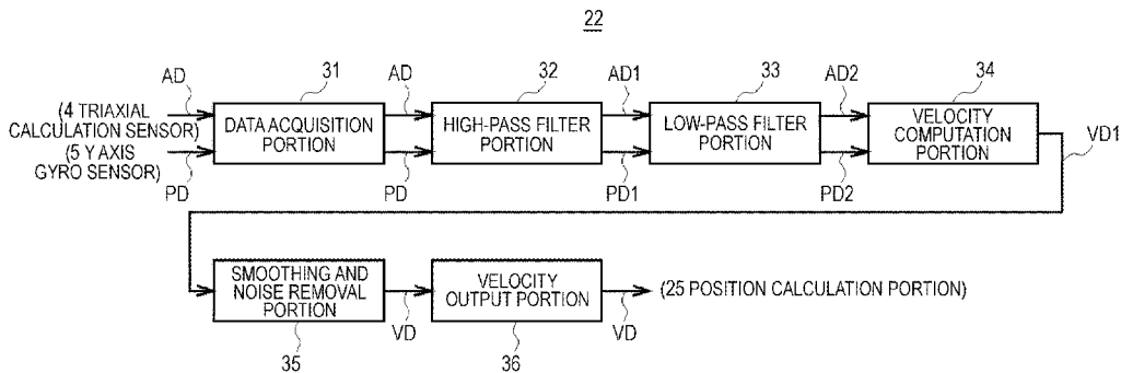
CONFIGURATION OF VELOCITY CALCULATION PORTION
