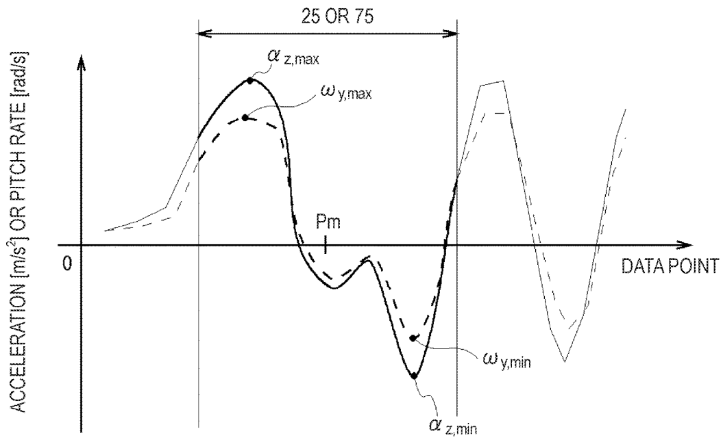
RELATION OF MAXIMUM VALUE AND MINIMUM VALUE
