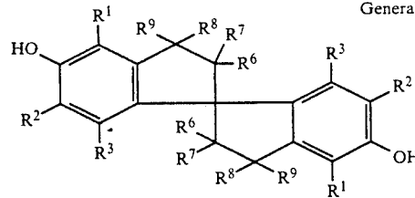
General Formula (G-3)
