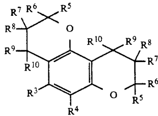
General Formula (F-5)
