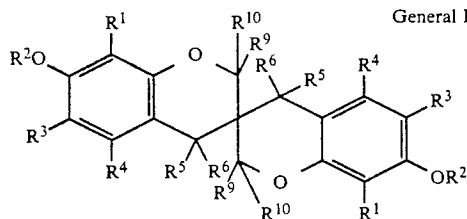
General Formula (B-5)
