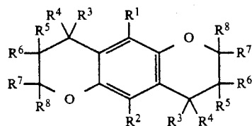
General Formula (C-2)
