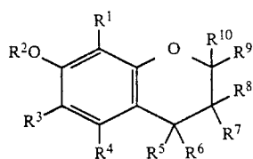
General Formula (B-2)
