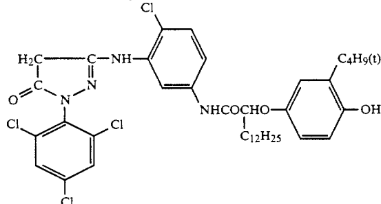
Comparative magenta coupler 3:
