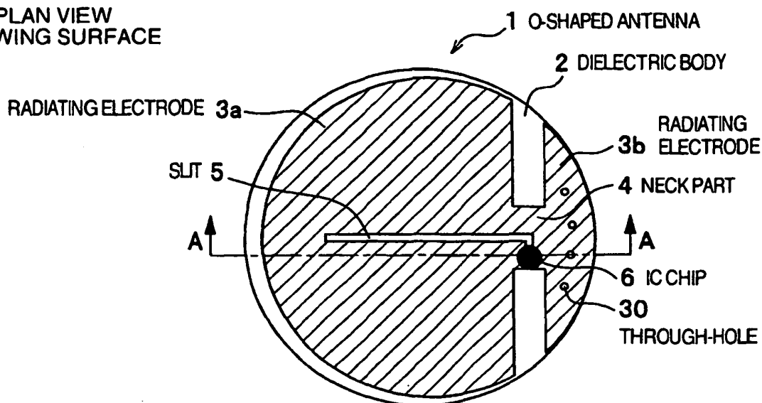
FIG.2B SECTIONAL VIEW TAKEN ALONG A-A
