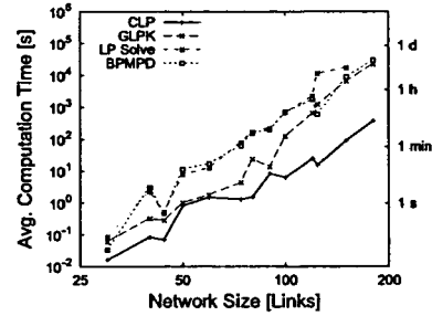
Fig. 5. Average computation time of the GLPK, BPMPD, CLP, and LPSolve for the optimization of different random networks depending on the network size in links only.
