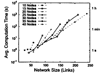
Fig. 9. Average computation time of the CLP for the optimization of different random networks depending on the network size in links and nodes.
