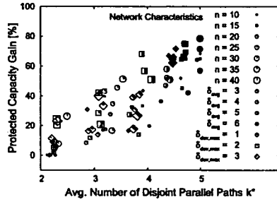
Fig. 4. Protected transmission gain of the SPM compared to SPR for random networks depending on their average number of average parallel paths.
