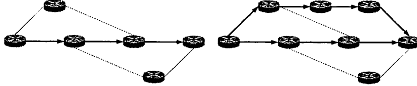
Fig. 2. The wrong selection of the first shortest path prohibits a another disjoint path.
