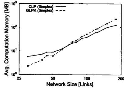
Fig. 8. Average memory consumption of the CLP and GLPK solvers for the optimization of different random networks depending on the network size in links only.
