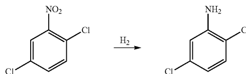
Scheme 5. Reaction scheme for the hydrogenation of 2,5-dichloronitrobenzene to 2,5-dichloroaniline.
