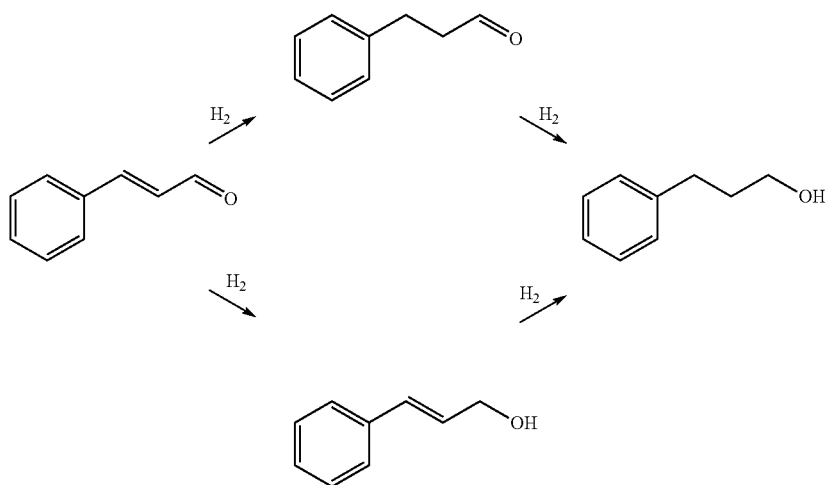
Scheme 3. Reaction scheme for the hydrogenation of cinnamaldehyde to hydrocinnamaldehyde, cinnamyl alcohol and 3-phenyl-1-propanol.
