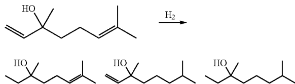
Scheme 4. Reaction scheme for the hydrogenation of linalool to 1,2-dihydrolinalool, 6,7-dihydrolinalool and 3,7-dimethyloctan-3-ol.
