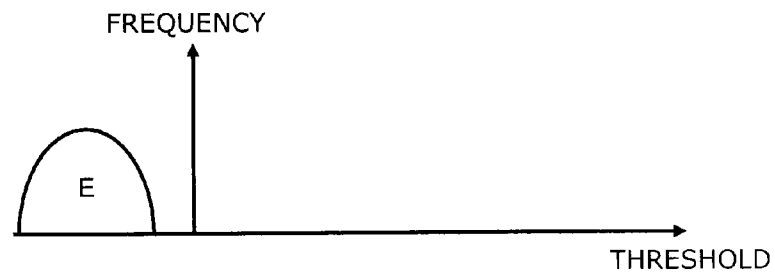
FIG. 4A ERASE STATE
