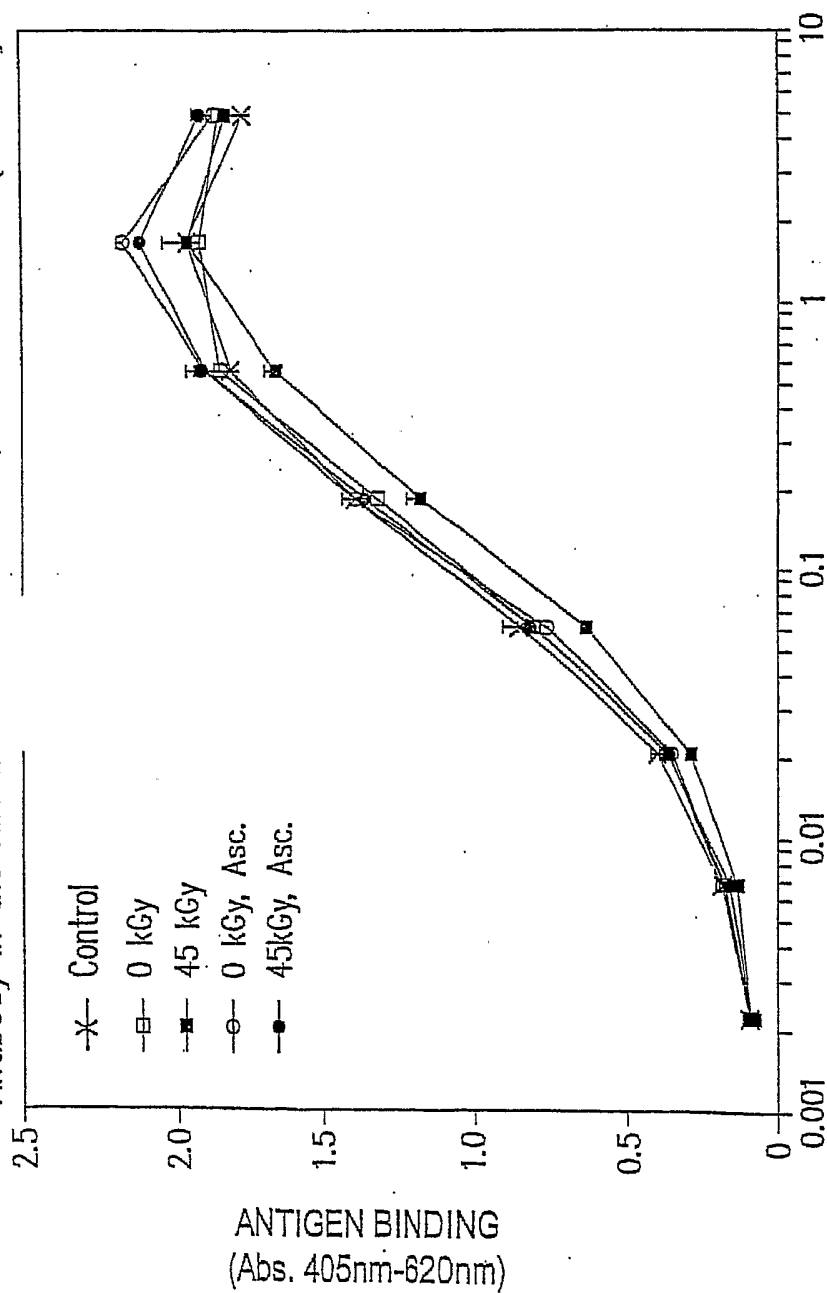
01.29.01 Gamma Irradiation of Freeze-dried Anti-Insulin Monoclonal Antibody in the Absence or Presence of 20mM Ascorbate (1% HSA)
