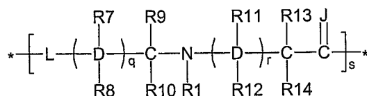
Structure II
