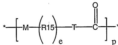
Structure II
