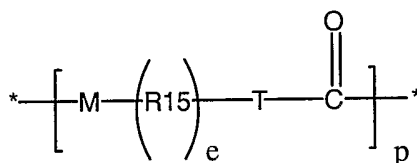
Structure III
