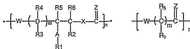
Structure I
