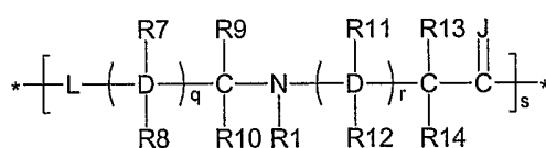
Structure II
