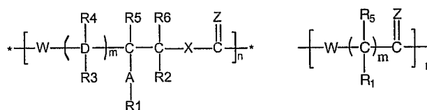
Structure I
